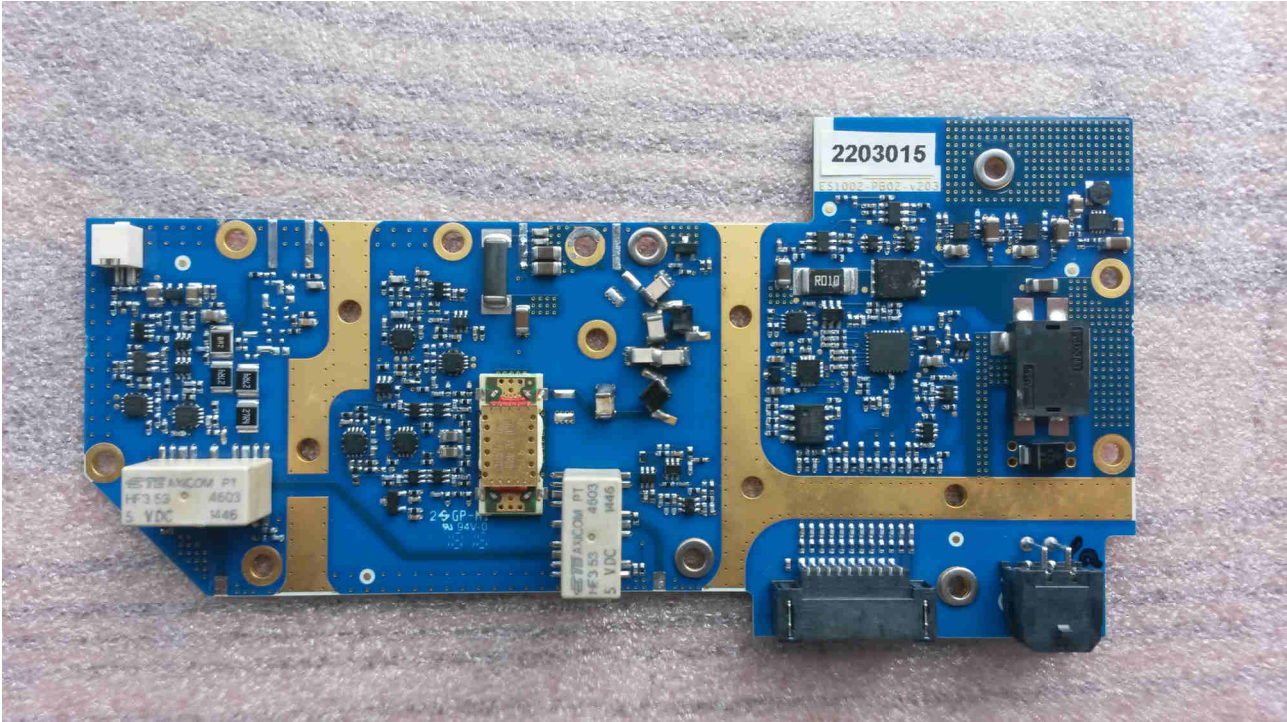
ES1002-PB02 UHF Low Power Amplifier PCB Assembly Top
