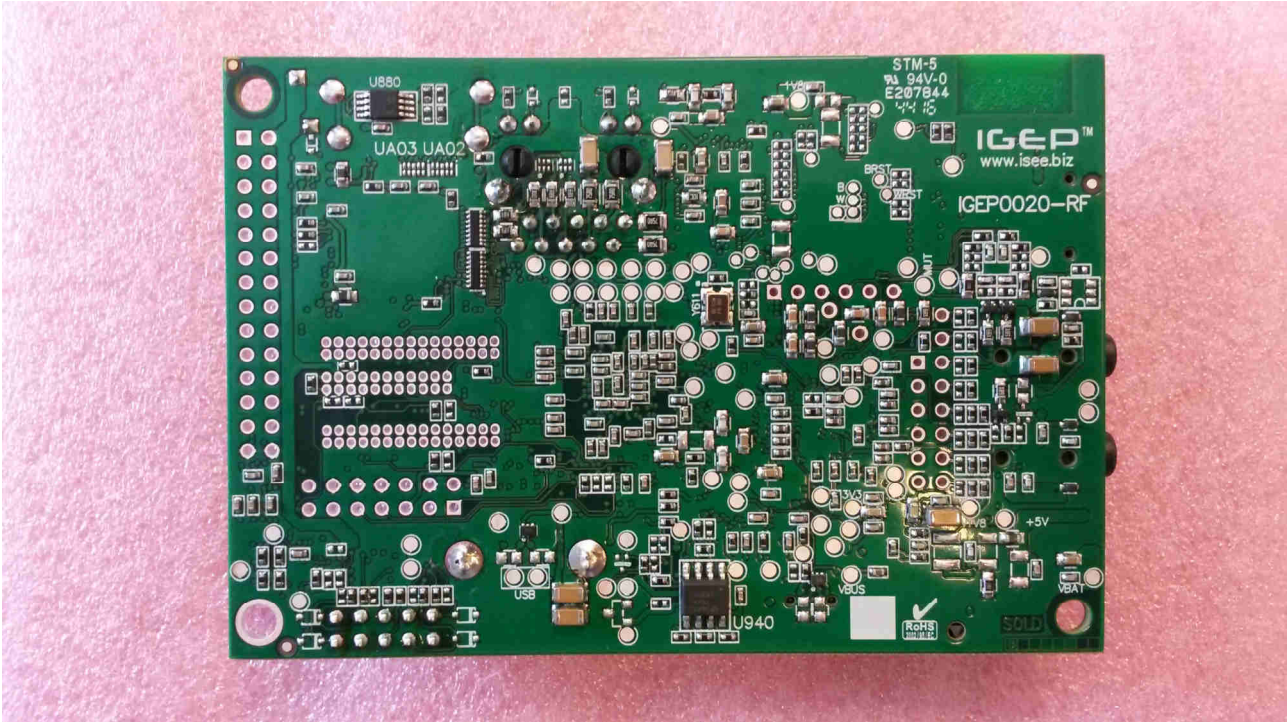
IGEP PCB Assembly Bottom
