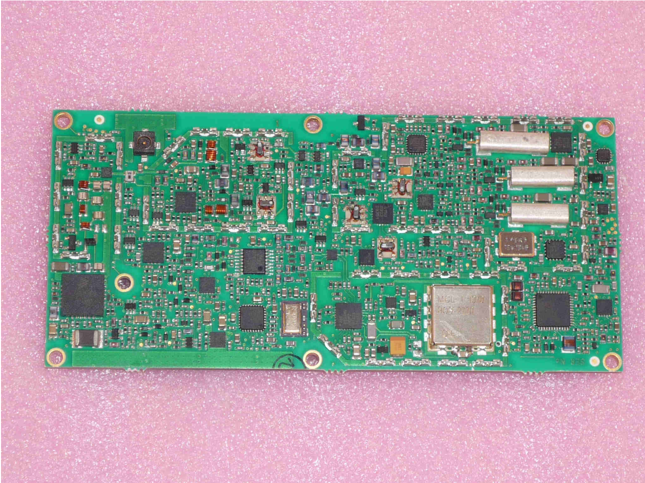
XR25 UHF Transceiver Top without Shields
