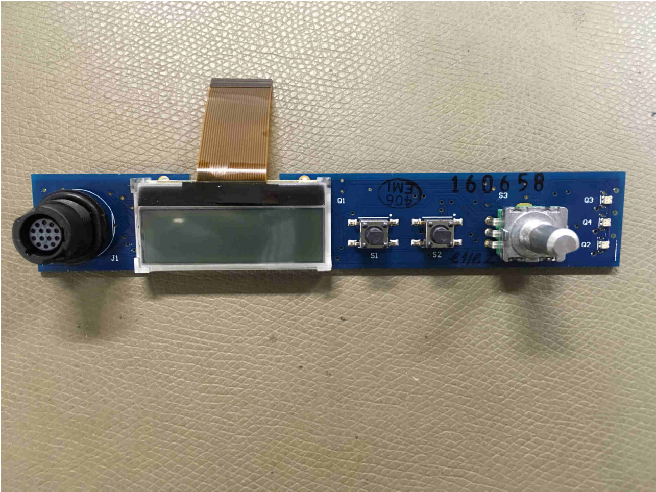
ES1002-PB06 Controller MMI PCB Assembly Top
