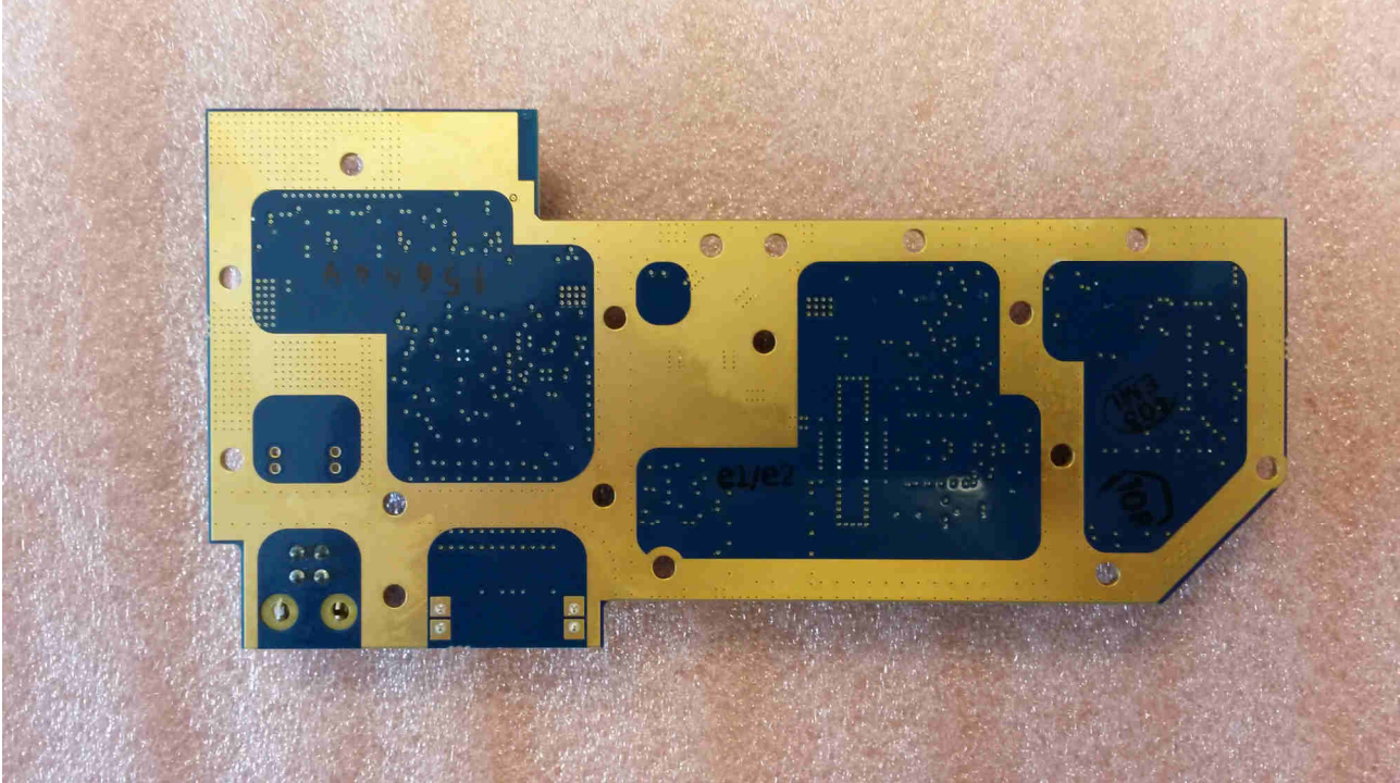
ES1002-PB02 UHF Low Power Amplifier PCB Assembly Bottom
