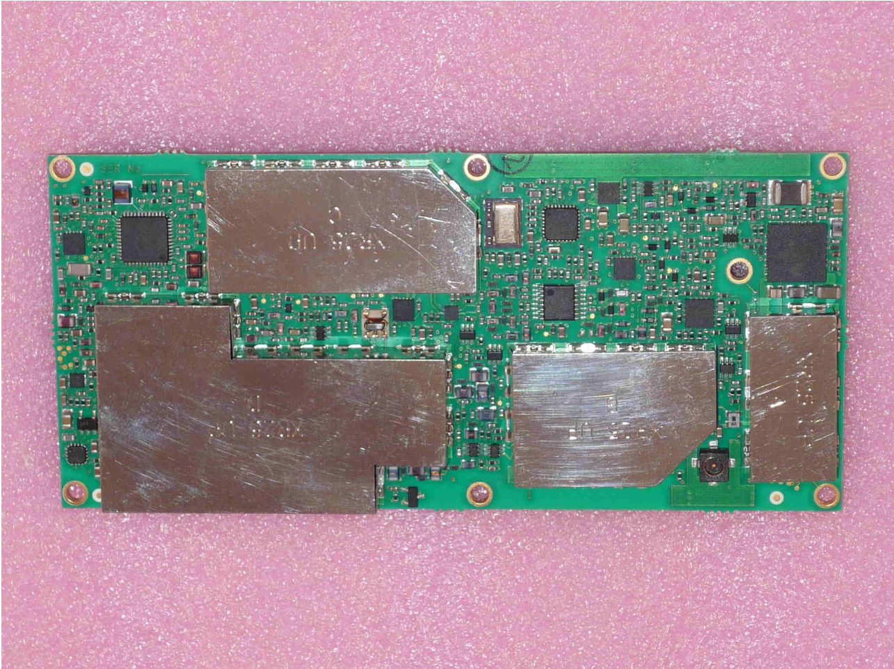
XR25 UHF Transceiver Top with Shields
