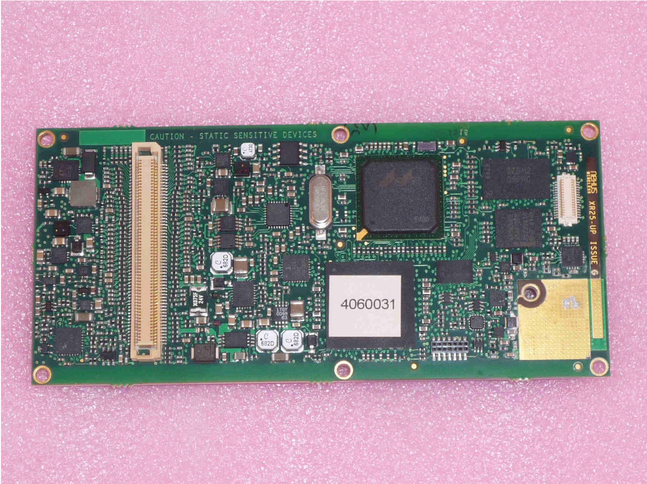
XR25 UHF Transceiver Bottom
