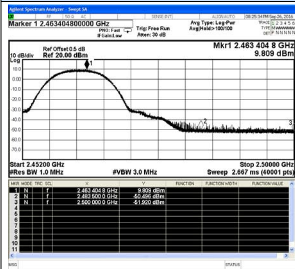
802.11b-High channel(Peak)
