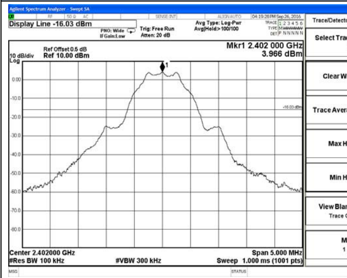
BT LE-Low channel Reference
