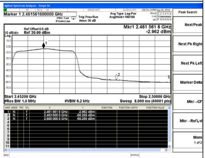
802.11n(HT20)-High channel(Average)
