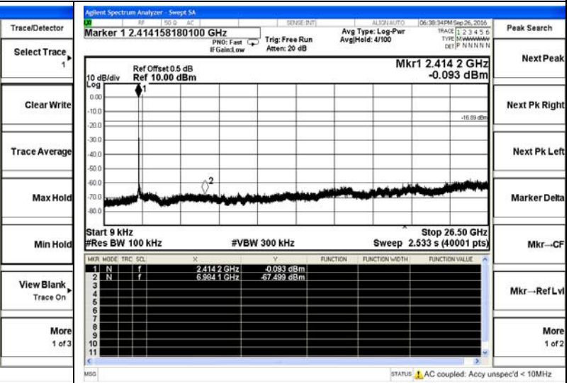
IEEE 802.11b-Low channel
