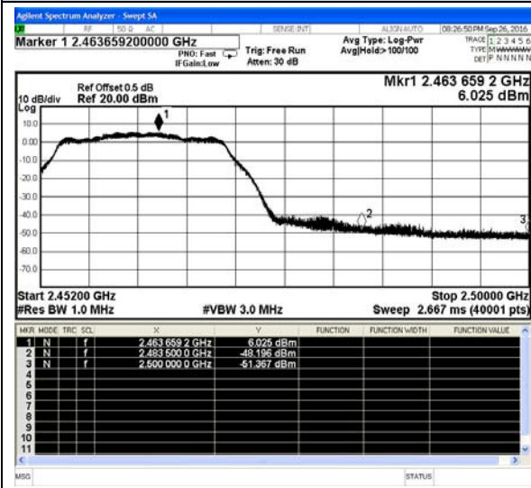
802.11g-High channel(Peak)
