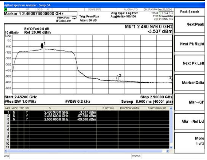
802.11g-High channel(Average)
