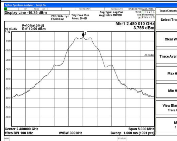
BT LE-High channel Reference
