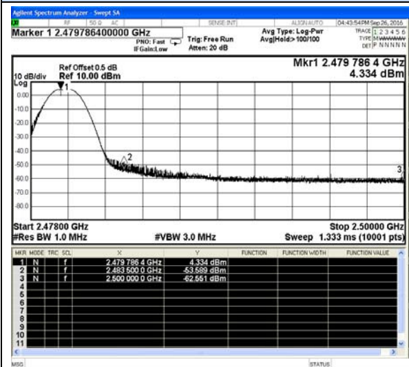
BT LE-High channel(Peak)
