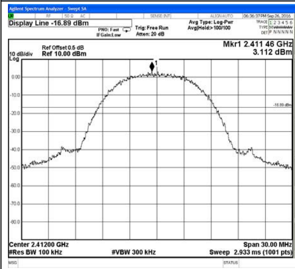
IEEE 802.11b-Low channel Reference
