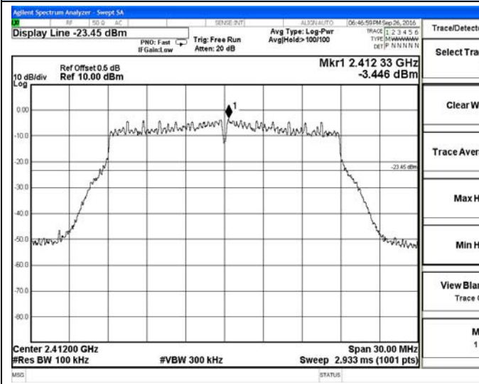
IEEE 802.11n(HT20)-Low channel Reference
