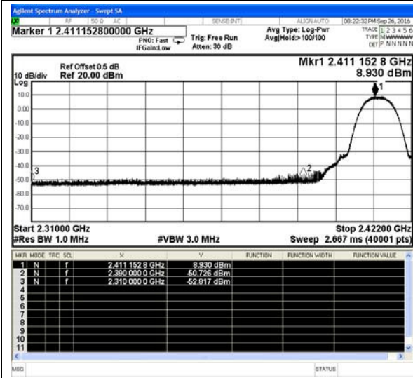
802.11b-Low channel(Peak)
