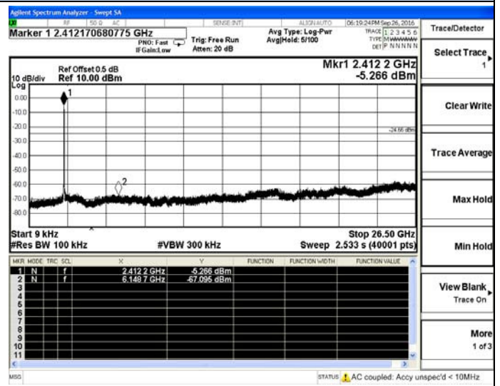
IEEE 802.11g-Low channel
