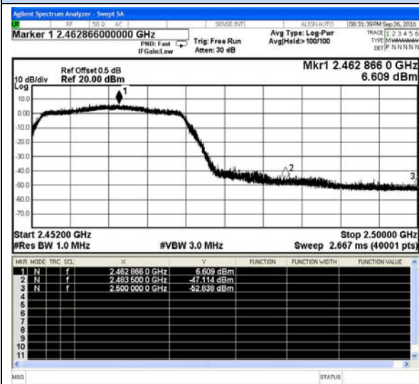
802.11n(HT20)-High channel(Peak)
