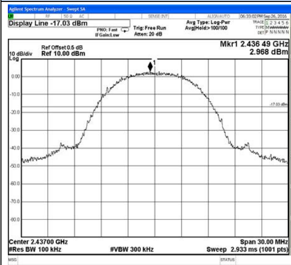
IEEE 802.11b-Middle channel Reference
