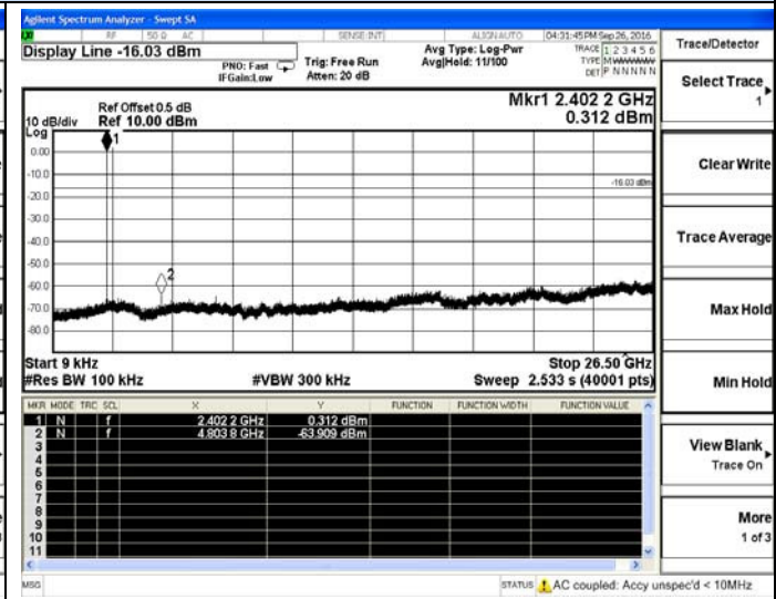
BT LE-Low channel
