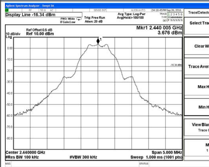
BT LE-Middle channel Reference
