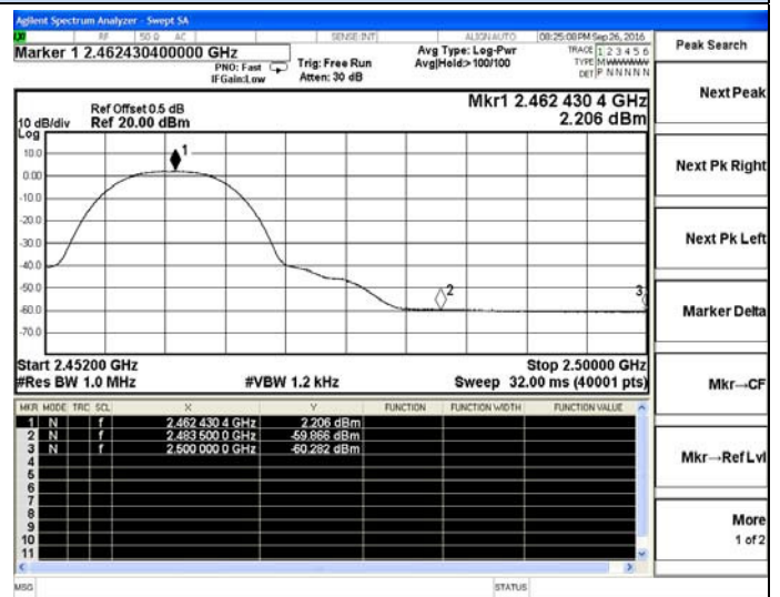
802.11b-High channel(Average)
