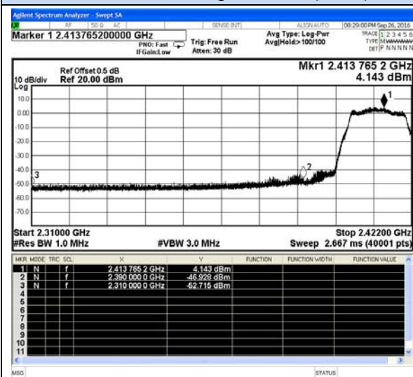
802.11g-Low channel(Peak)
