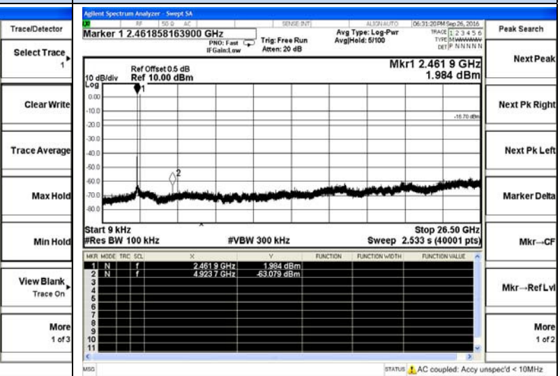
IEEE 802.11b-High channel
