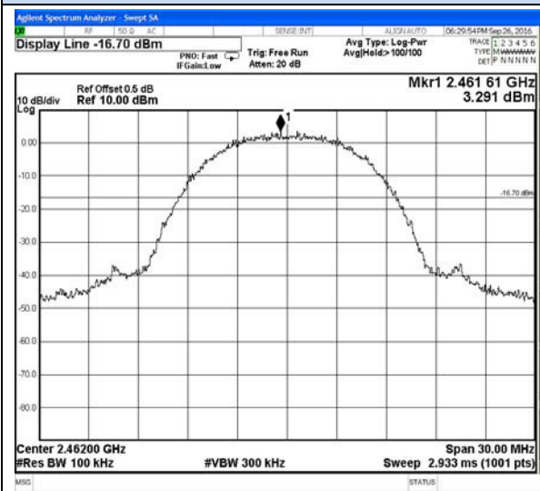
IEEE 802.11b-High channel Reference
