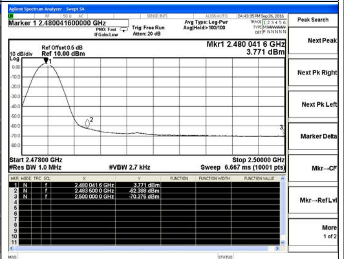
BT LE-High channel(Average)
