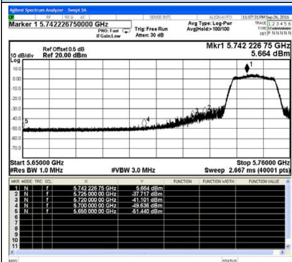
802.11ac20-Low channel(Peak)
