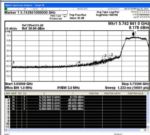
802.11a-Low channel(Peak)
