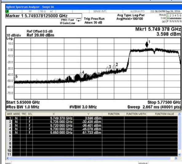
802.11n-HT40-Low channel(Peak)
