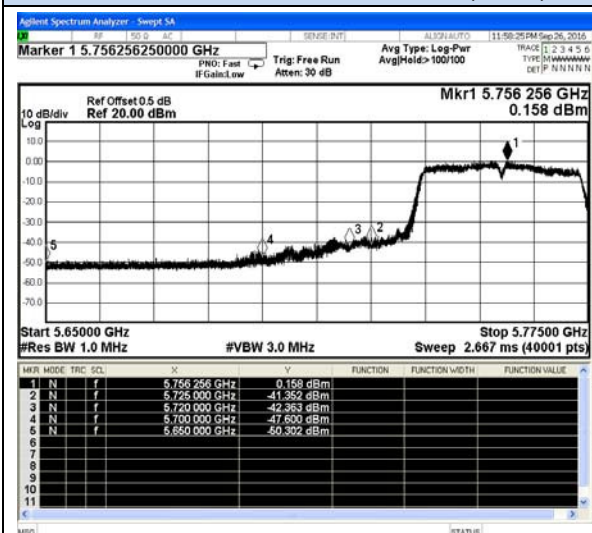
802.11ac40-Low channel(Peak)
