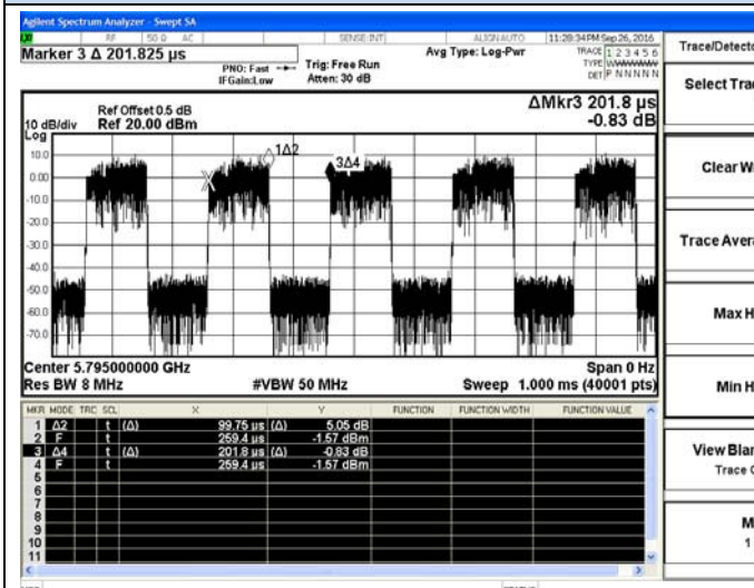
802.11n-HT40
