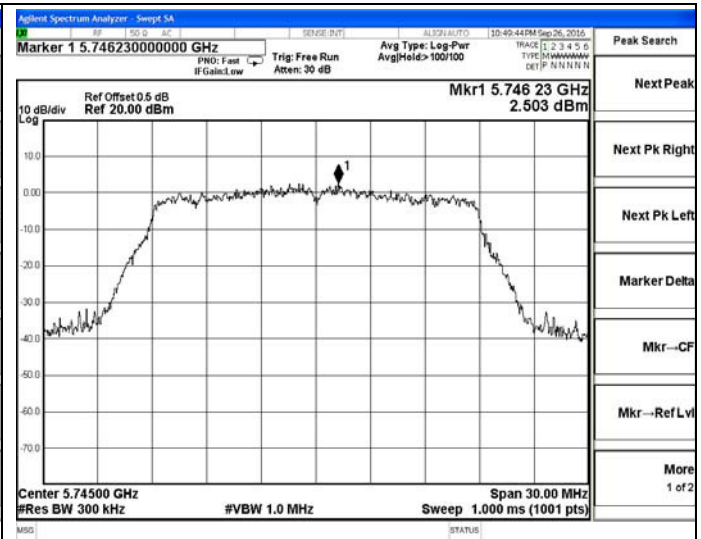
802.11ac20-5745MHz
