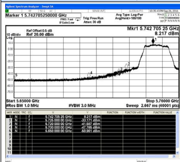
802.11n-HT20-Low channel(Peak)
