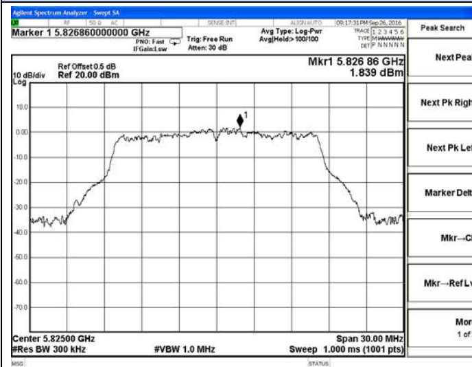
802.11a-5825MHz
