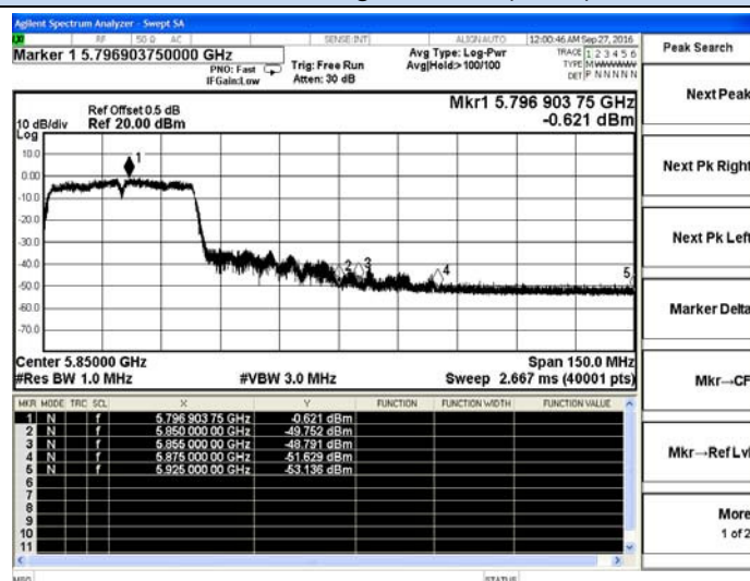
802.11ac40-High channel(Peak)
