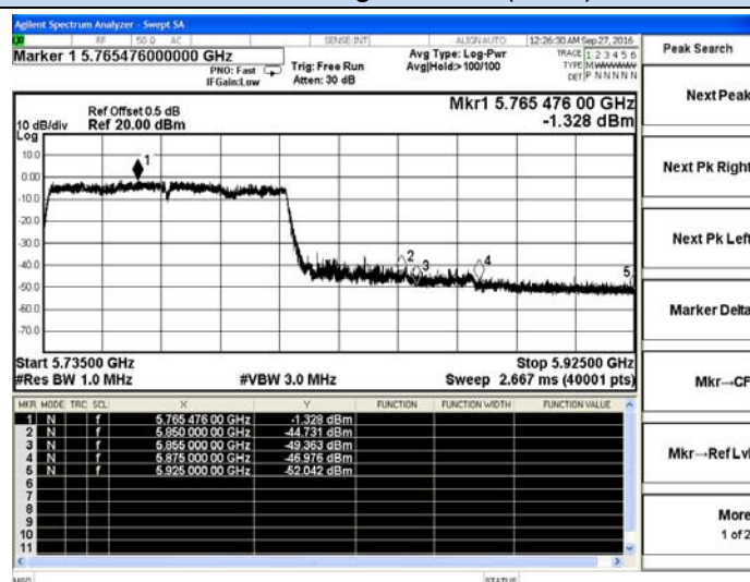
802.11ac80-High channel(Peak)
