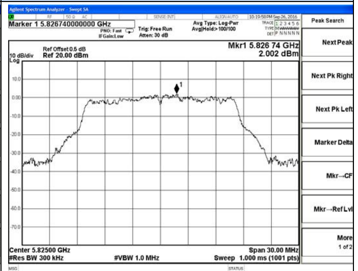
802.11n-HT20-5825MHz
