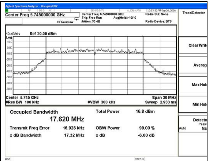
802.11ac20-5745MHz
