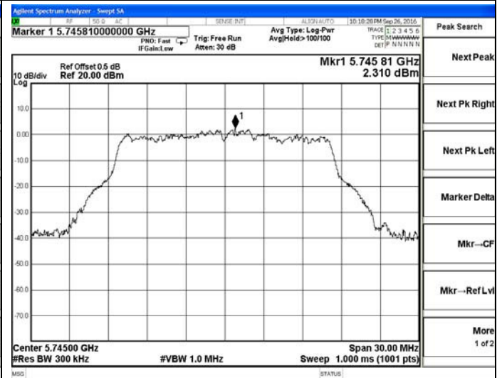
802.11n-HT20-5745MHz
