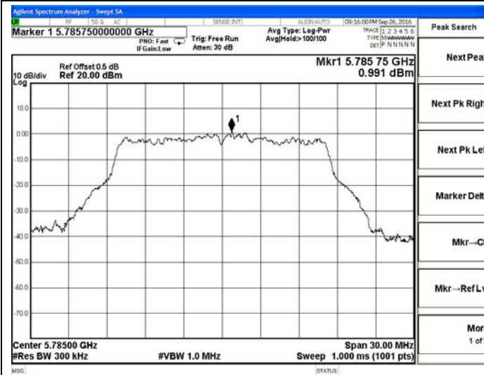
802.11a-5785MHz
