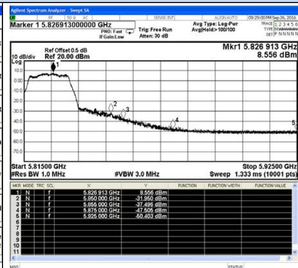
802.11a-High channel(Peak)
