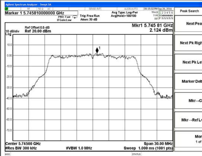
802.11a-5745MHz
