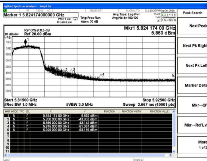
802.11ac20-High channel(Peak)
