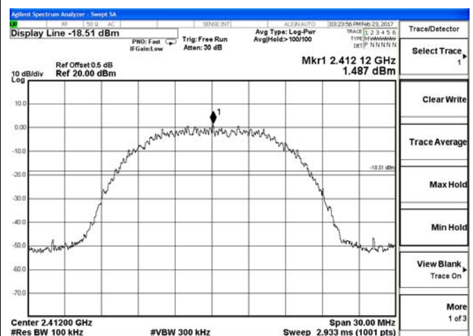
802.11b_Low Channel
