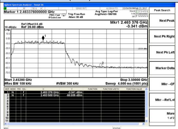
802.11n(HT20)-High channel
