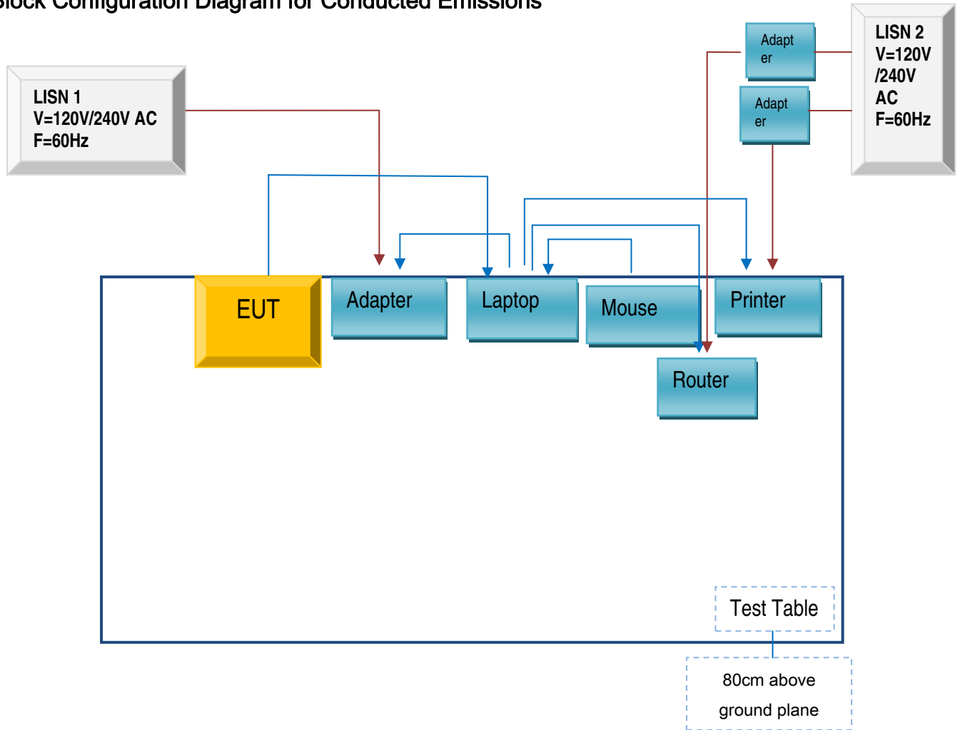
Block Configuration Diagram for Conducted Emissions
