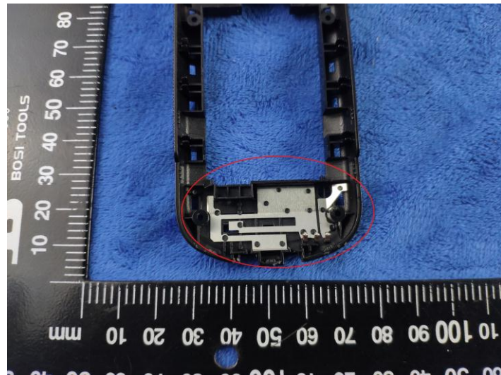
GSM/PCS/UMTS Antenna
