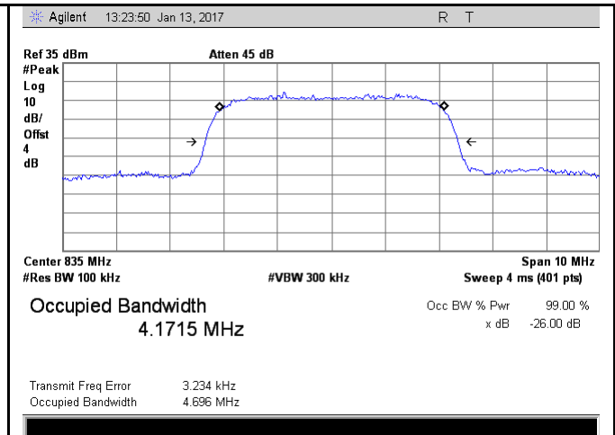
Band V BW - Mid CH 835.0 MHz
