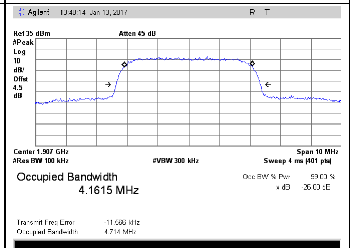
Band II BW - High CH 1907.6MHz
