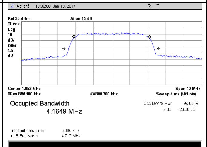
Band II BW - Low CH 1852.4MHz
