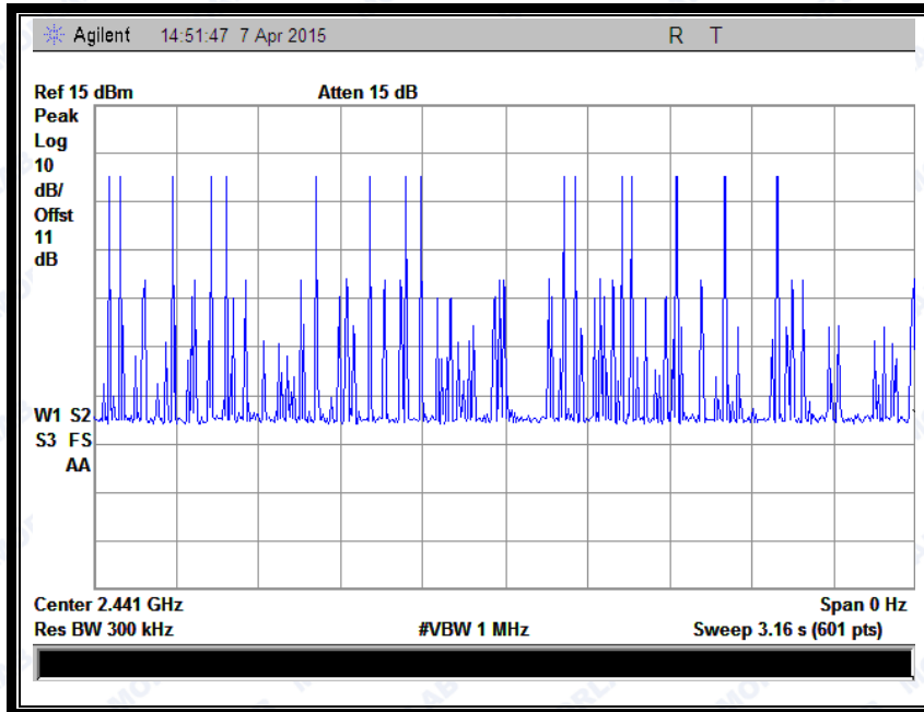
(Plot B: DH3 @ GFSK)
