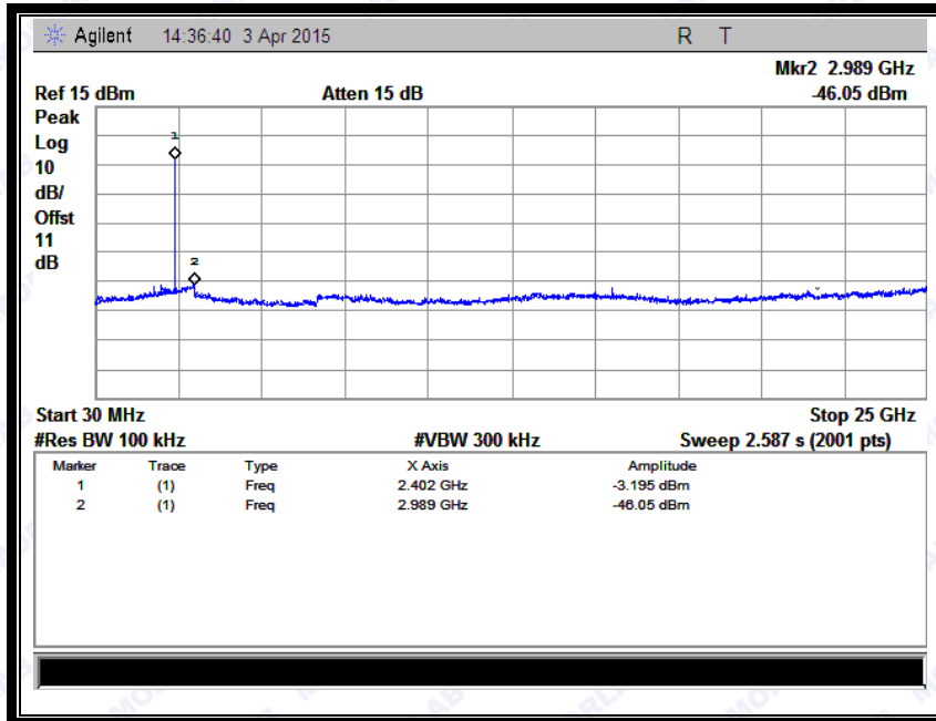
(Plot G.1: Channel = 0, 30MHz to 25GHz @ 8-DPSK)
