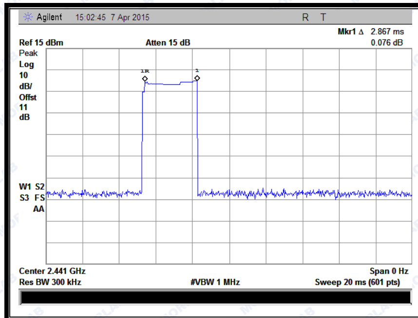
(Plot H: DH3 @ 8-DPSK)
