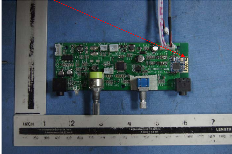
BT Antenna
