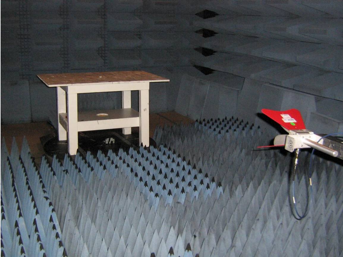
Radiated emissions test setup above 1000MHz
