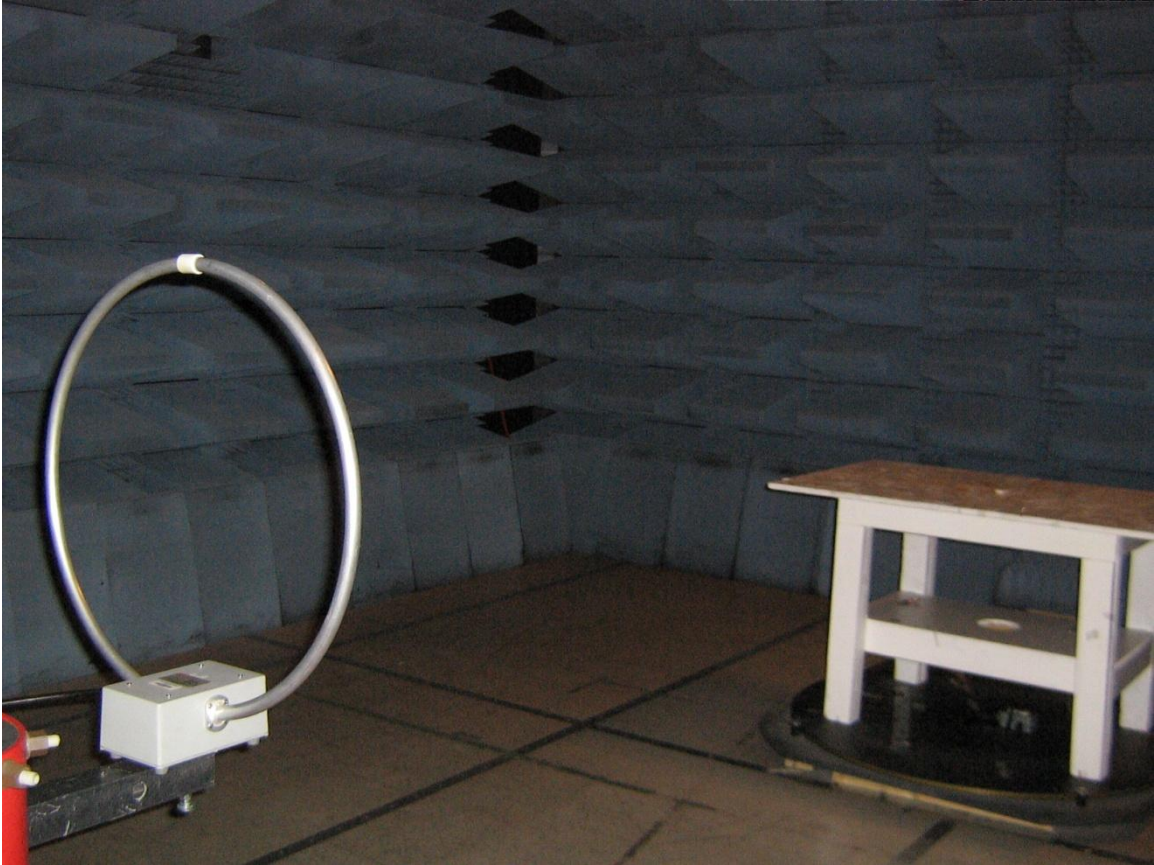
Radiated emissions test setup below 30MHz
