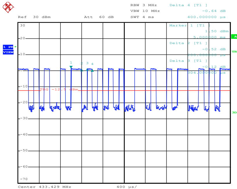
Pulse Time, 433.42MHz
