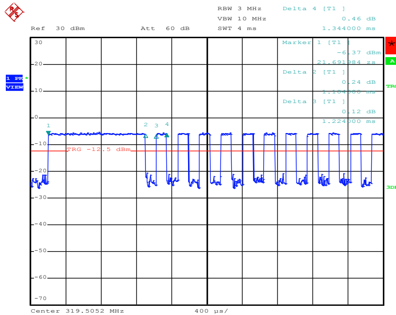
Pulse Time, 319.5MHz
