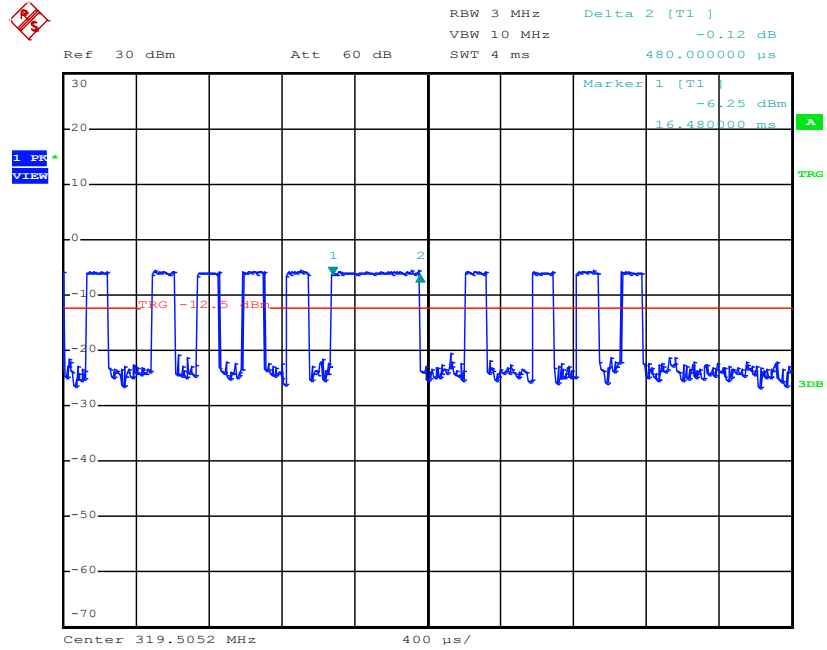
Mid Pulse Time, 319.5MHz
