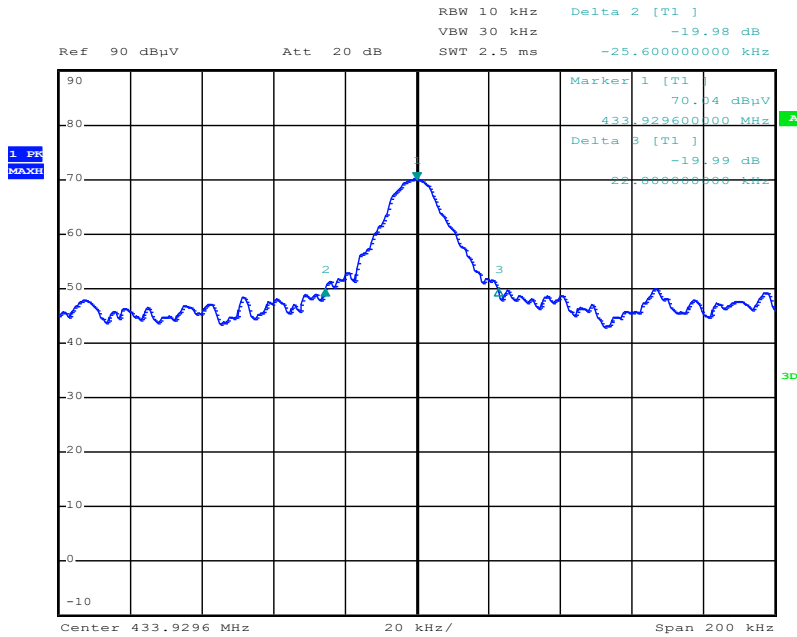
20 dB Occupied Bandwidth, 433.92 MHz
