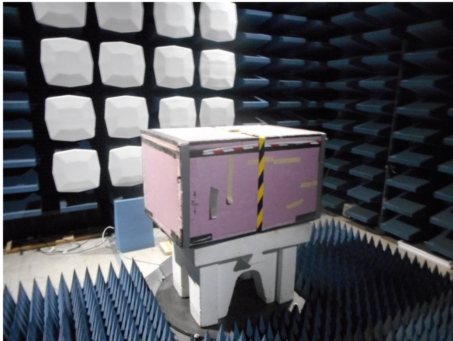
Radiated Emissions Above 1 GHz at the 3m SAC, EUT setup
