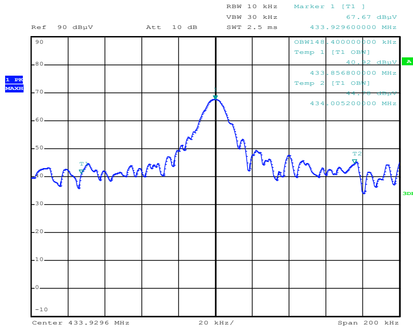
99% Occupied Bandwidth, 433.92 MHz
