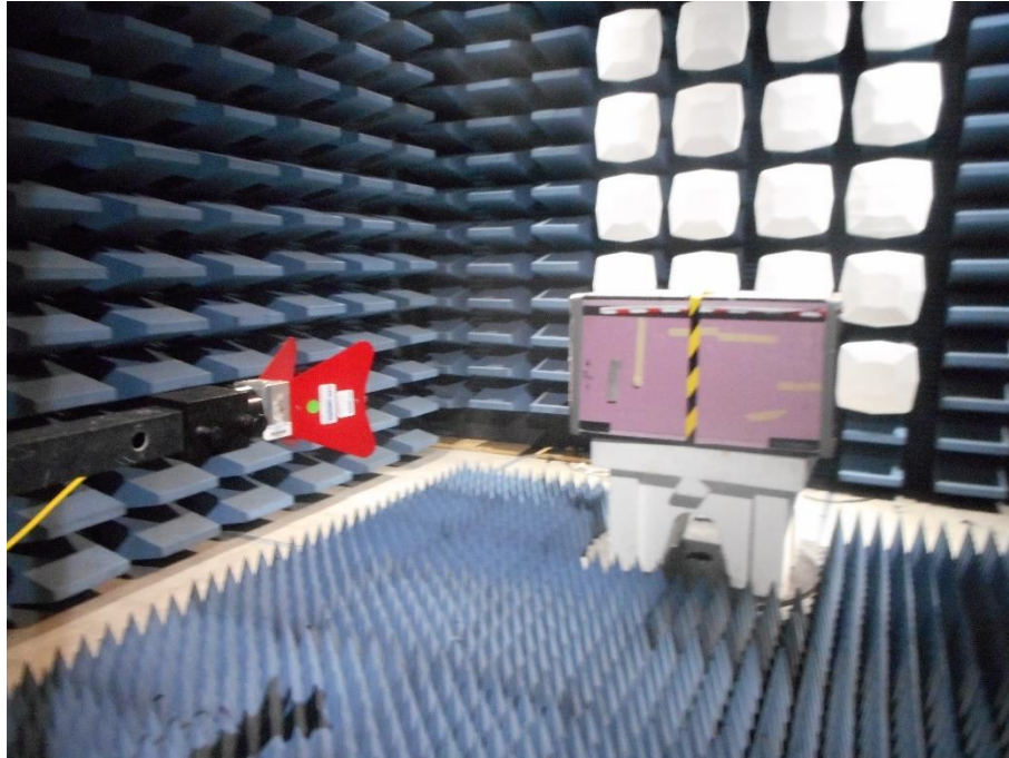
Radiated Emissions Above 1 GHz at the 3m SAC
