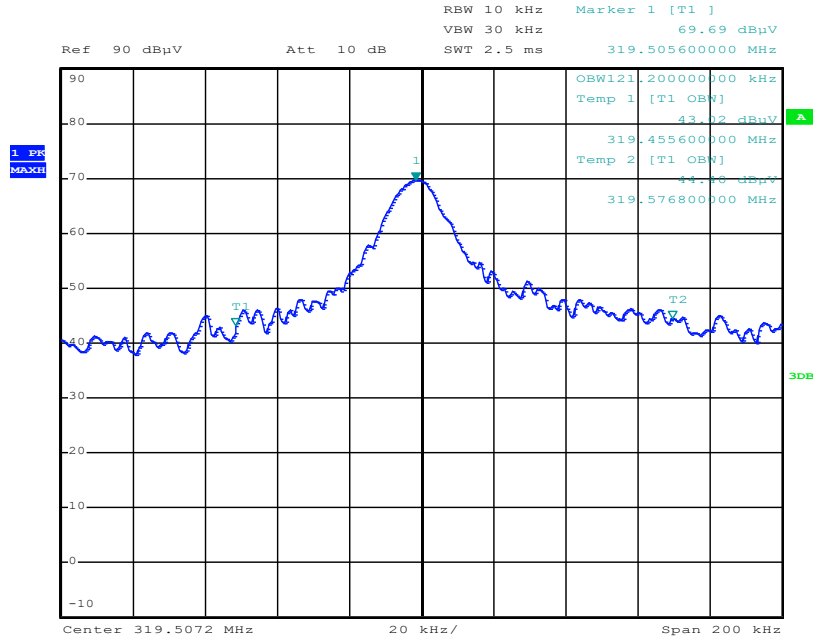
99% Occupied Bandwidth, 319.5 MHz
