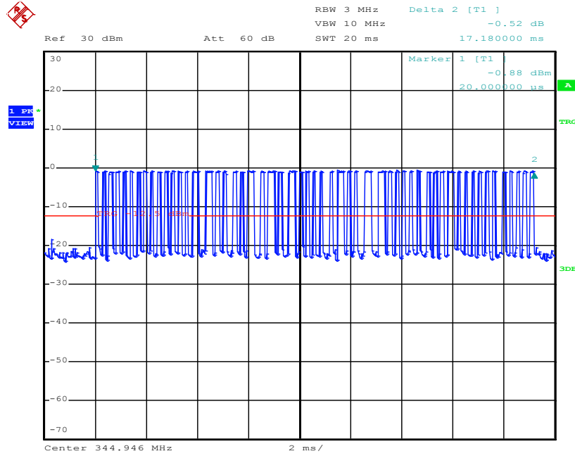
Pulse Number, 344.92MHz
