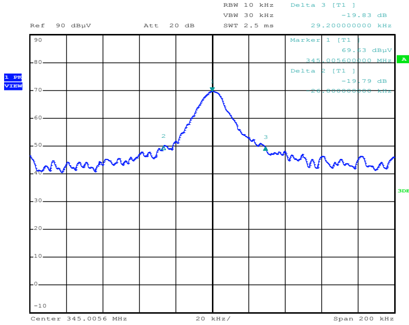
20 dB Occupied Bandwidth, 345 MHz
