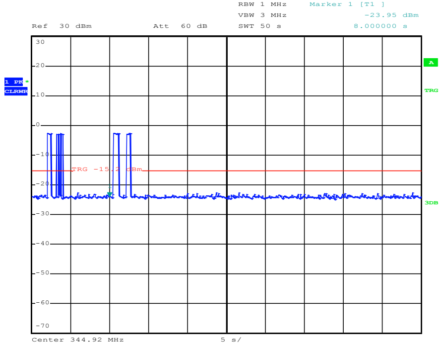
Transmission Time, 344.92MHz
