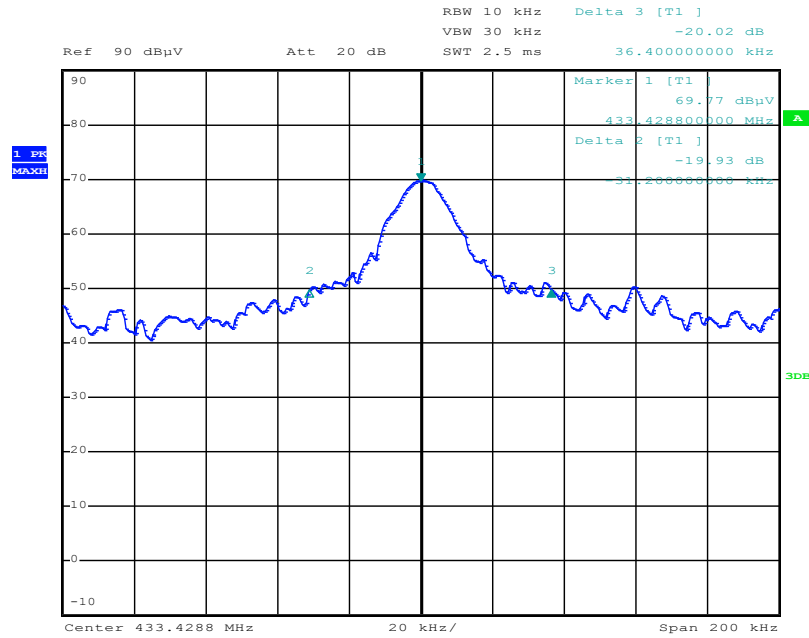
20 dB Occupied Bandwidth, 433.42 MHz
