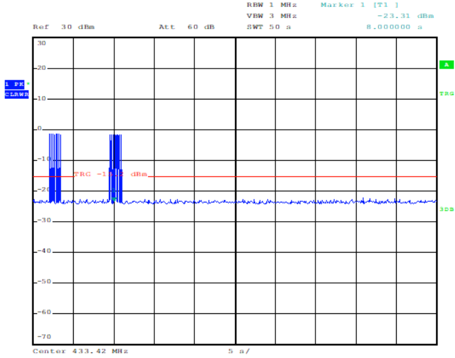
Transmission Time, 433.42MHz
