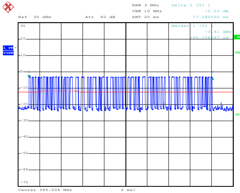
Pulse Number, 345MHz
