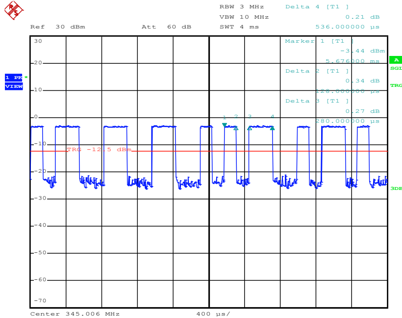
Pulse Time, 345MHz
