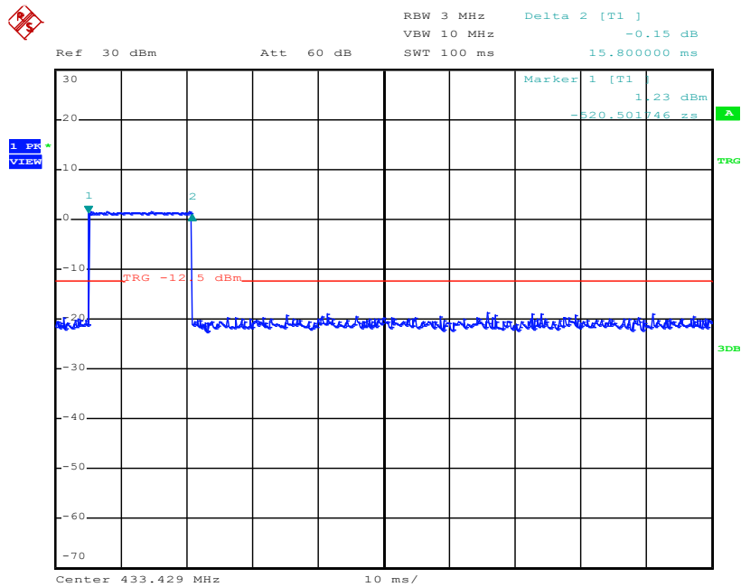
Transmissions Burst Duration In 100 ms, 433.42MHz
