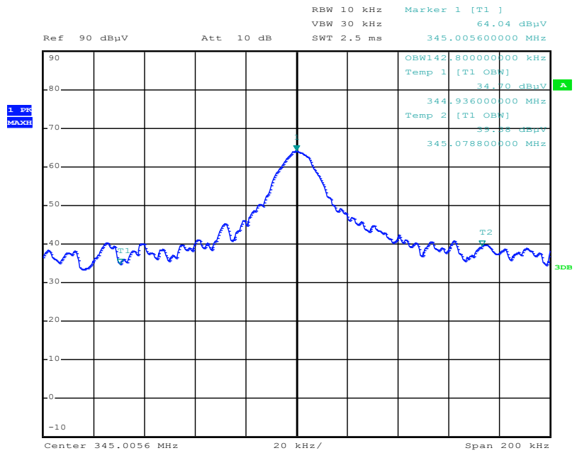
99% Occupied Bandwidth, 345 MHz
