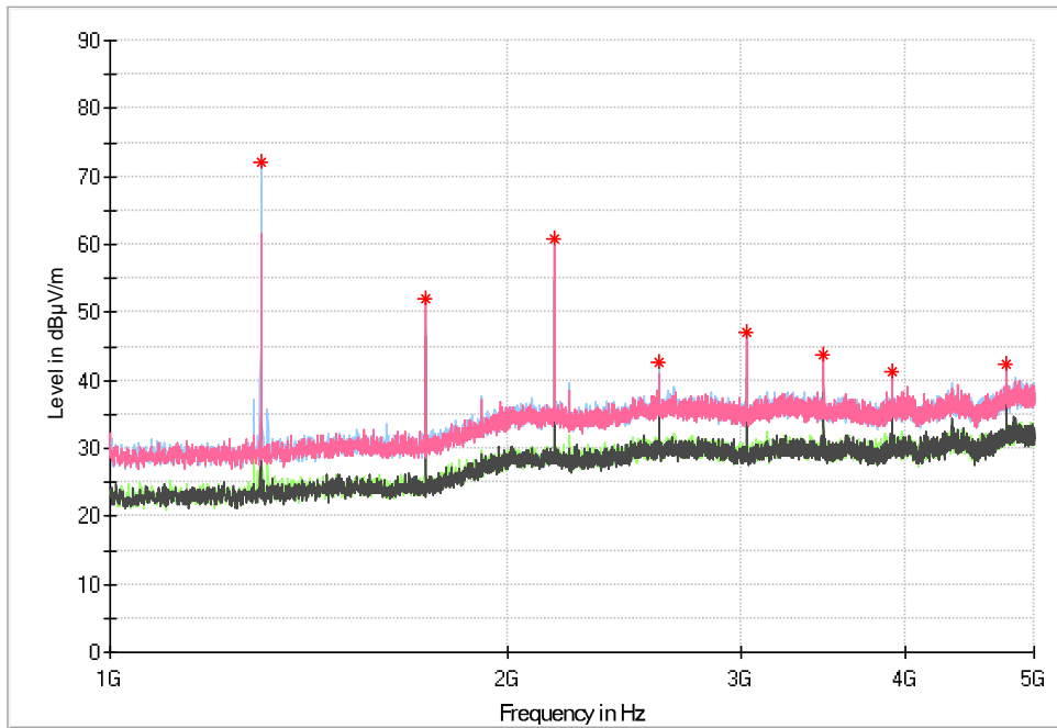
Radiated Emissions (1GHz-5GHz) scanned at 3m SAC
