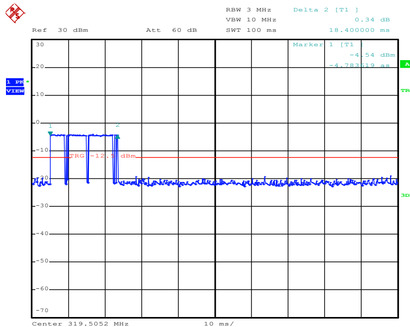
Transmissions Burst Duration In 100 ms, 319.5 MHz
