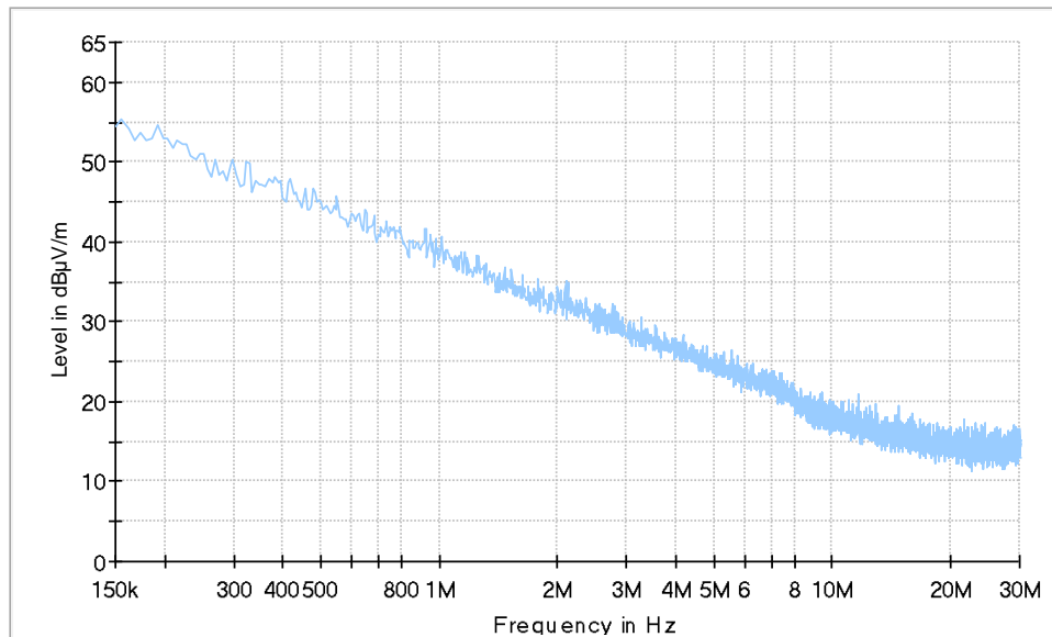
Radiated Emissions (150 kHz-30MHz) scanned at 3m SAC
