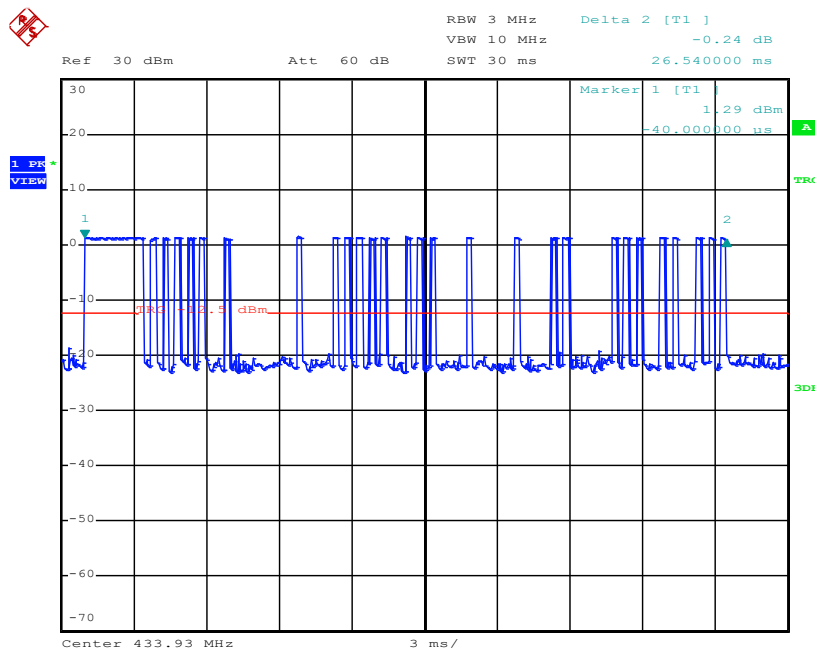
Pulse Number, 433.92MHz
