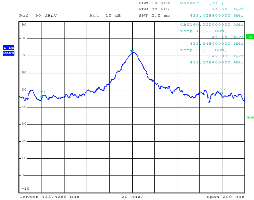
99% Occupied Bandwidth, 433.42 MHz
