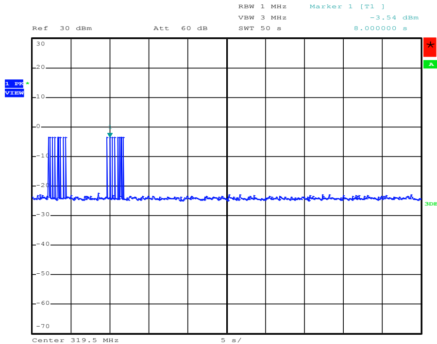
Transmission Time, 319.5MHz
