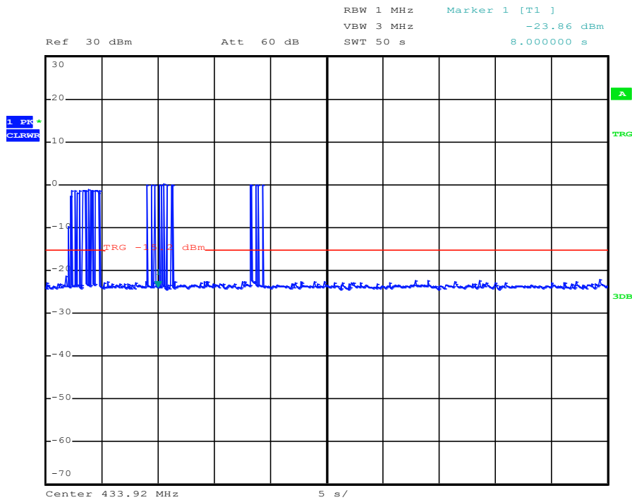
Transmission Time, 433.92MHz
