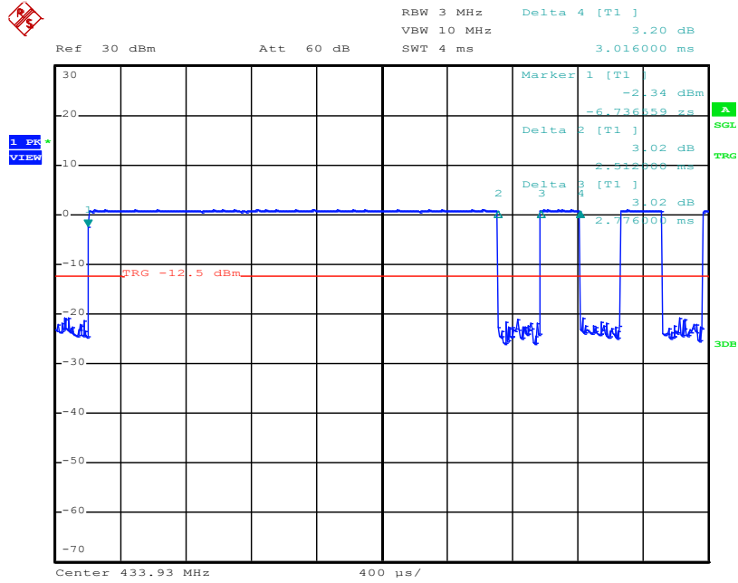
Pulse Time, 433.92MHz
