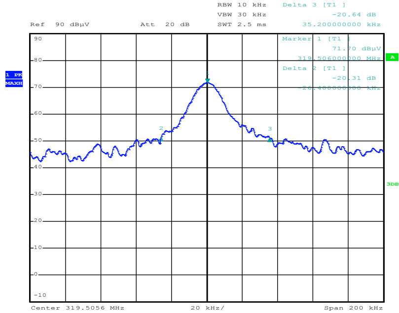
20 dB Occupied Bandwidth, 319.5 MHz
