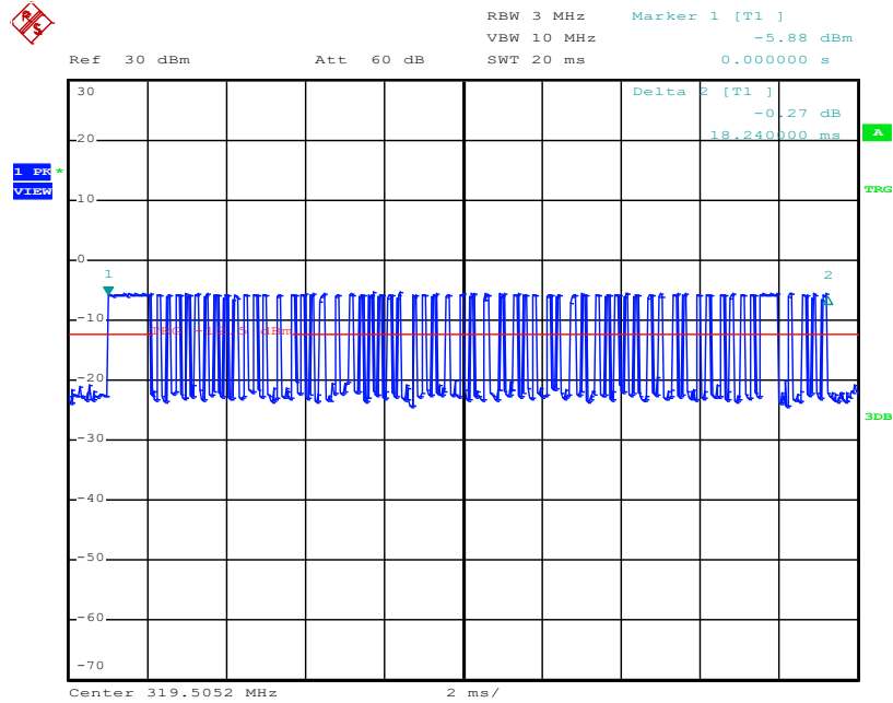
Pulse Number, 319.5MHz
