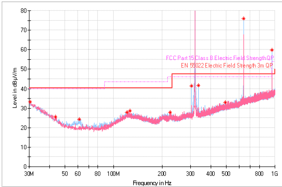
Radiated Emissions (30MHz-1GHz) scanned at 3m SAC
