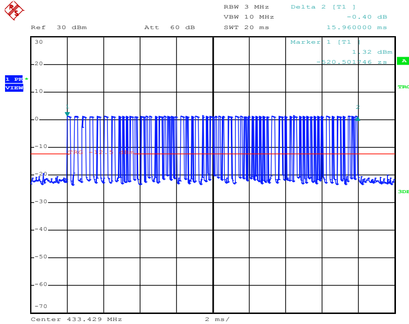
Pulse Number, 433.42MHz
