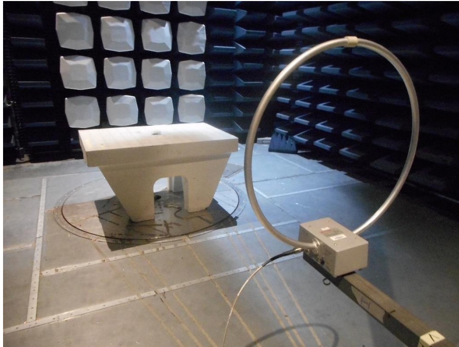
Radiated Emissions below 30 MHz at the 3m SAC
