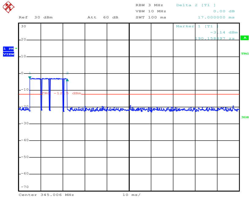
Transmissions Burst Duration In 100 ms, 345MHz
