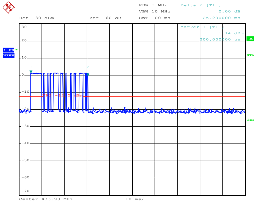
Transmissions Burst Duration In 100 ms, 433.92MHz
