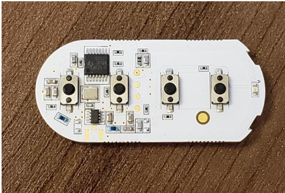
KFG Top Side of PCB
