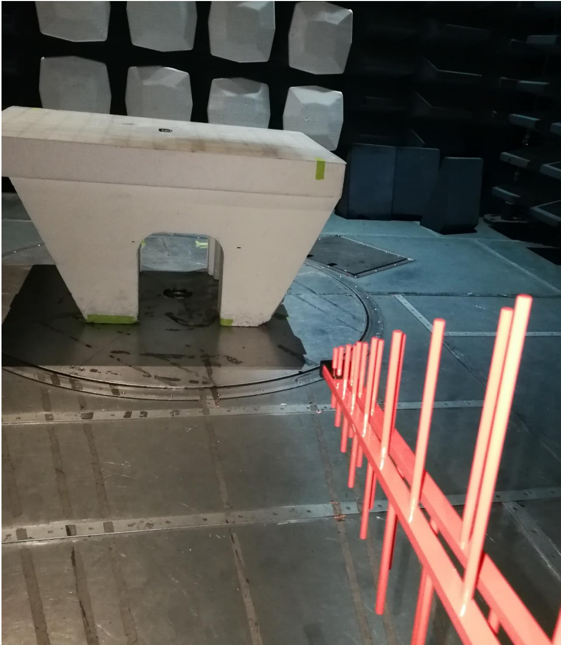
Figure 1: SAC Radiated Spurious Emissions (30 MHz – 1 GHz) at 3m
