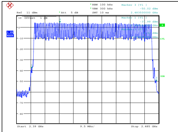
8-DPSK Hopping off 2480
