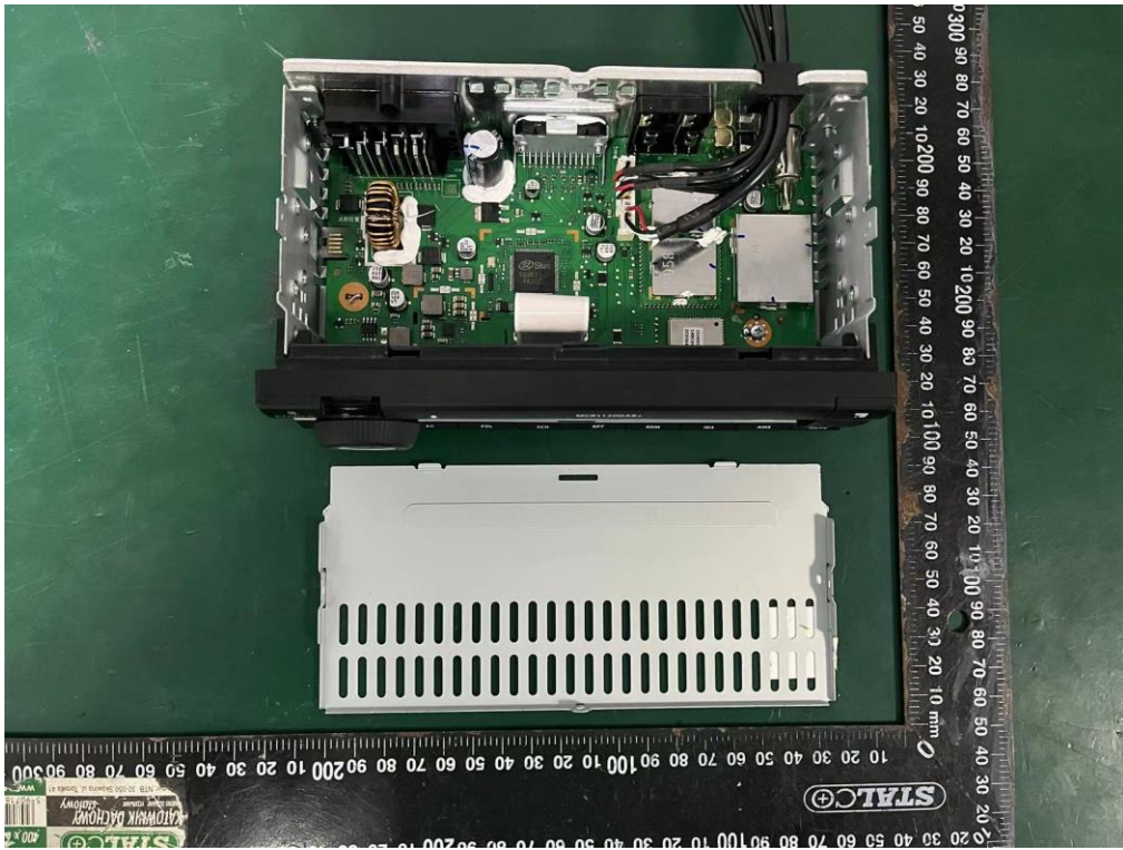
Internal photos M/N: MCR1120DAB+
