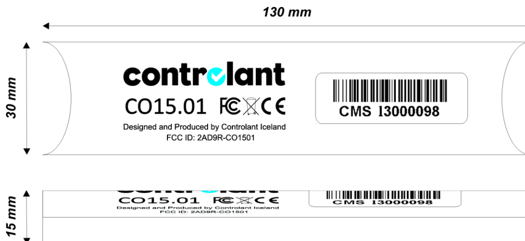
Figure 1: Mechanical drawing of the CO 15.01 wireless logger
