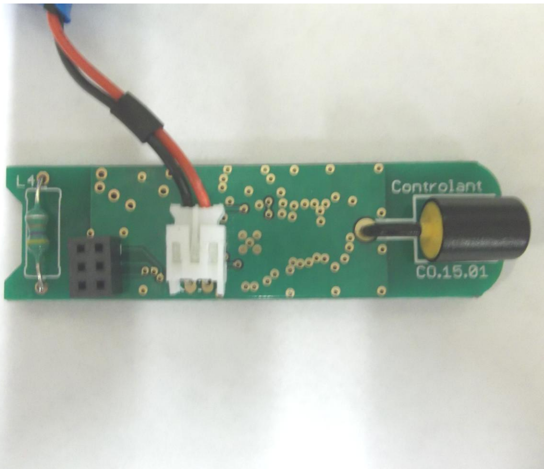
Figure 2. Back of EUT (antenna soldered to PCB)
