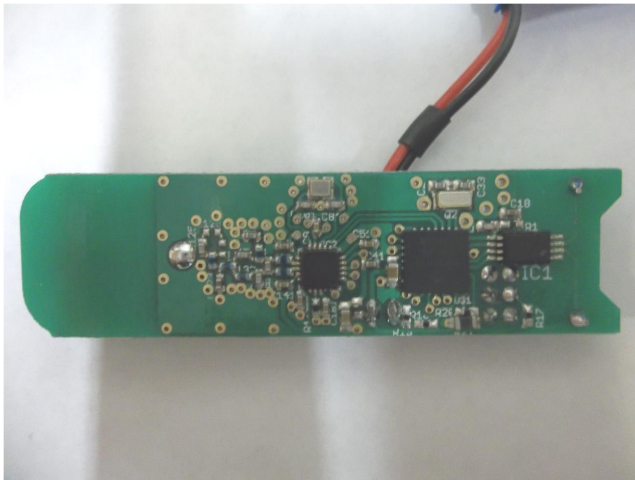
Figure 3. Front of EUT with Radio
