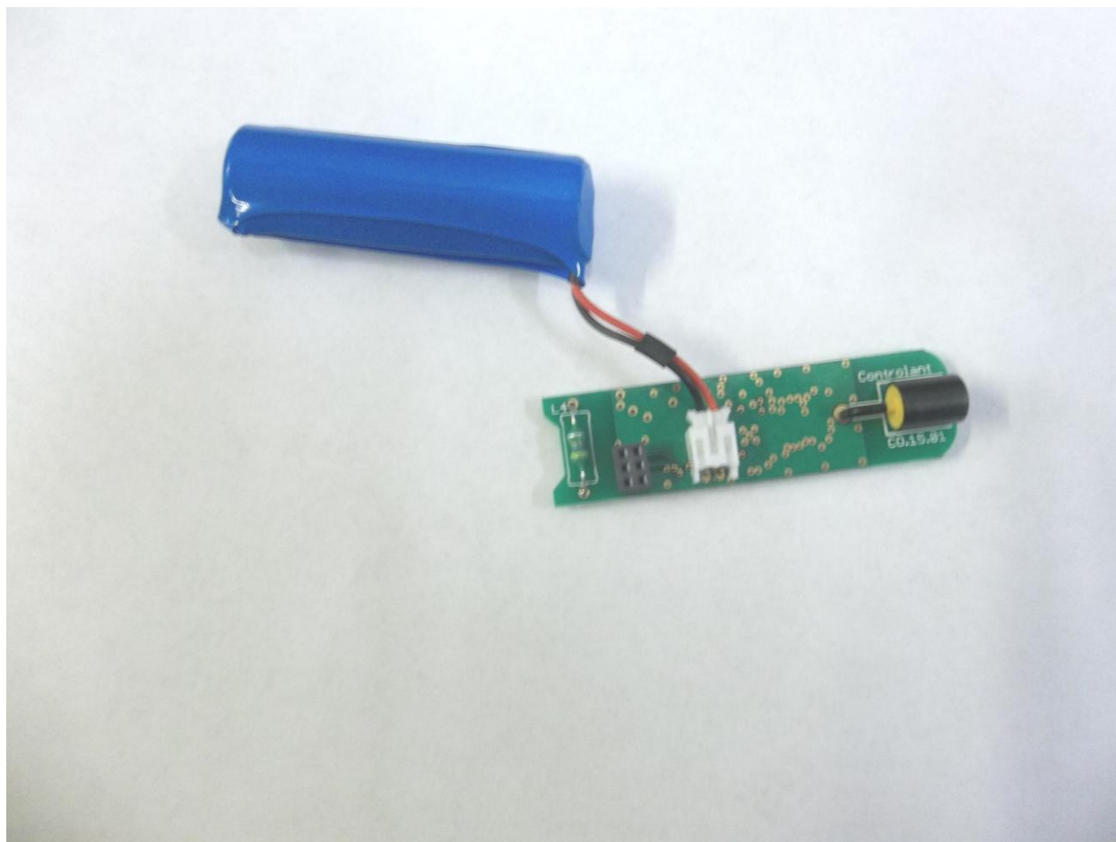
Figure 1. EUT with Case Removed
