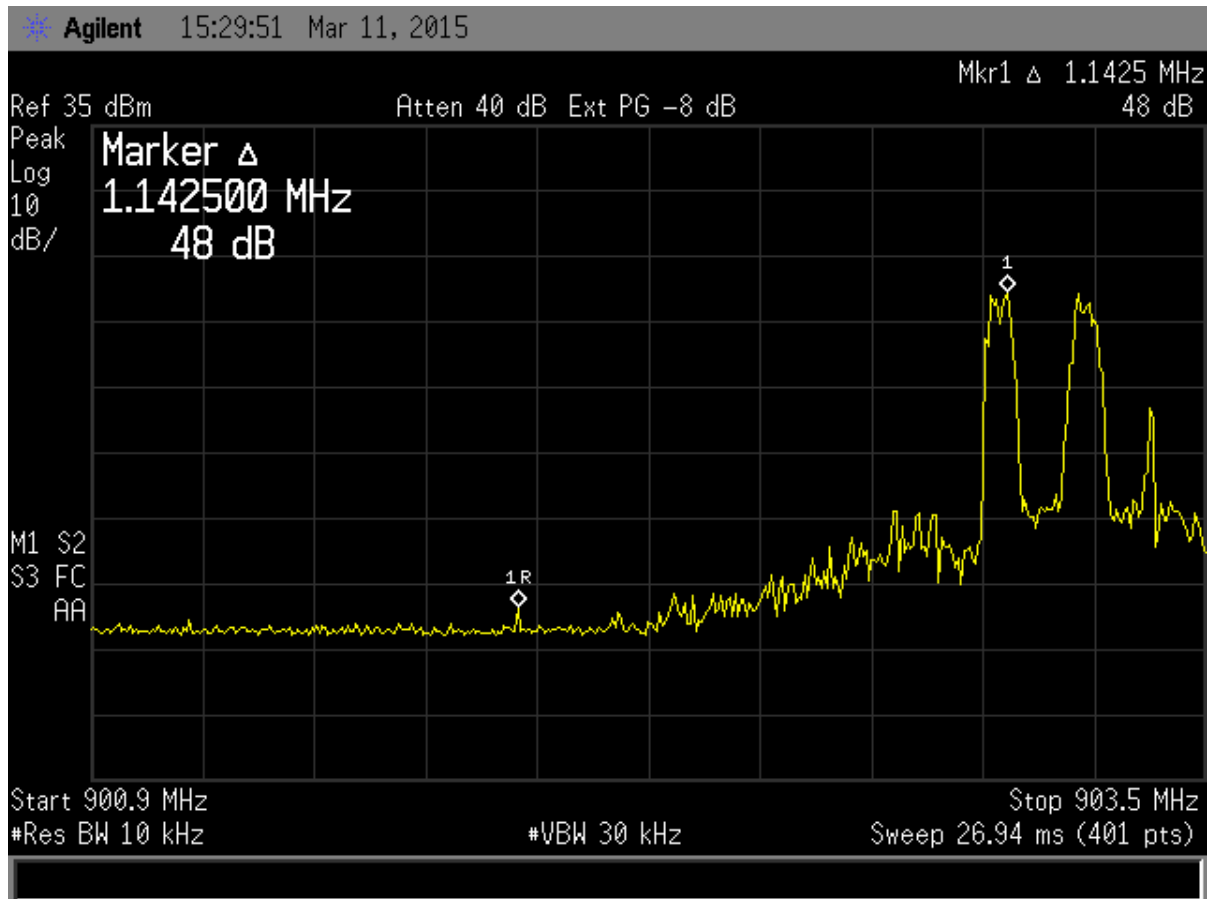
Figure 13. Band Edge Compliance, Low Channel Delta – Channel Hopping GFSK Modulation
