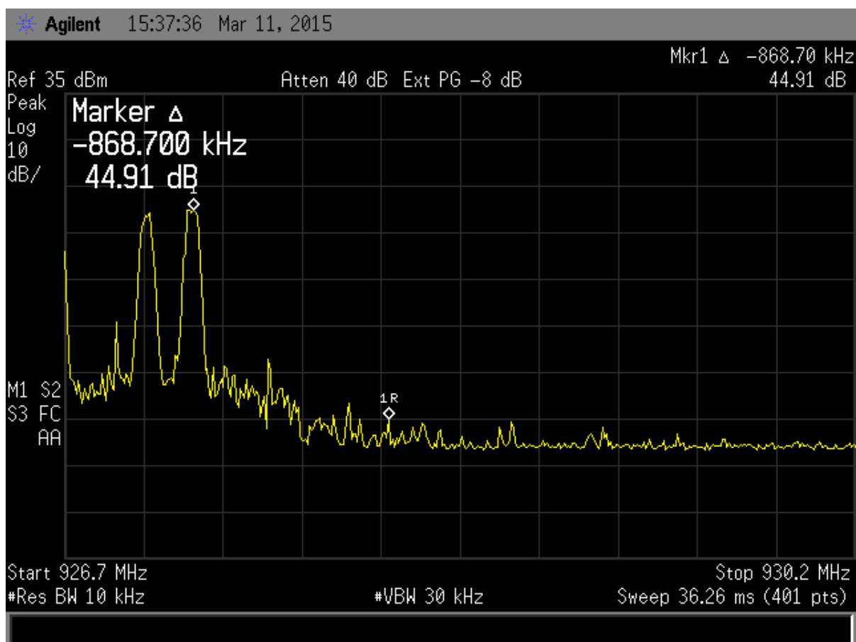
Figure 15. Band Edge Compliance, High Channel Delta – Channel Hopping GFSK Modulation
