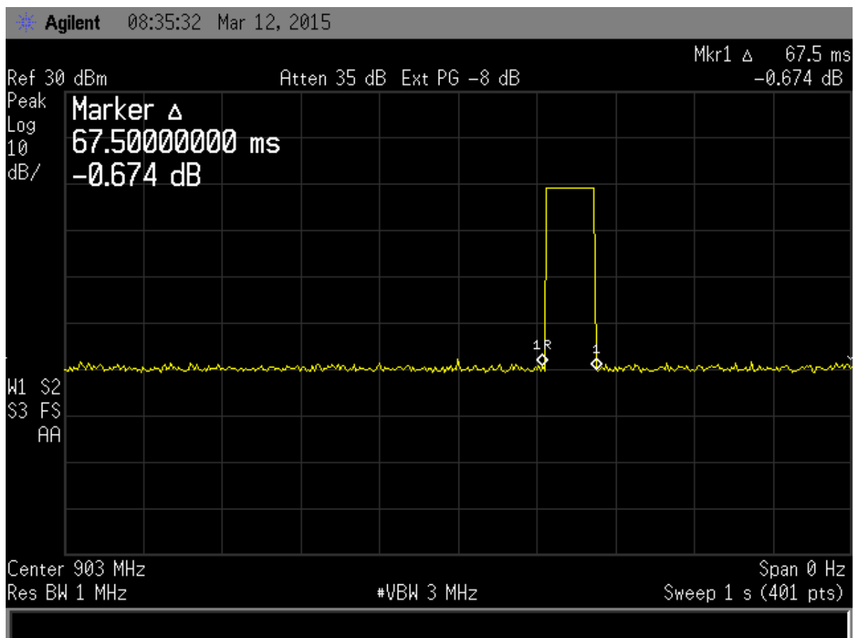
Figure 2. Transmitter Pulse Width in 1 Sec Period
