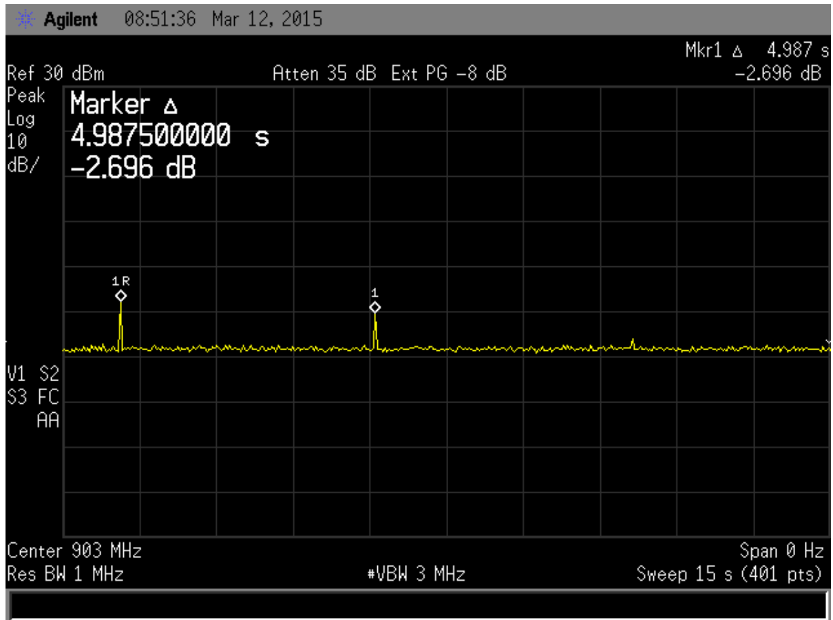
Figure 35. Time between Occupancy
