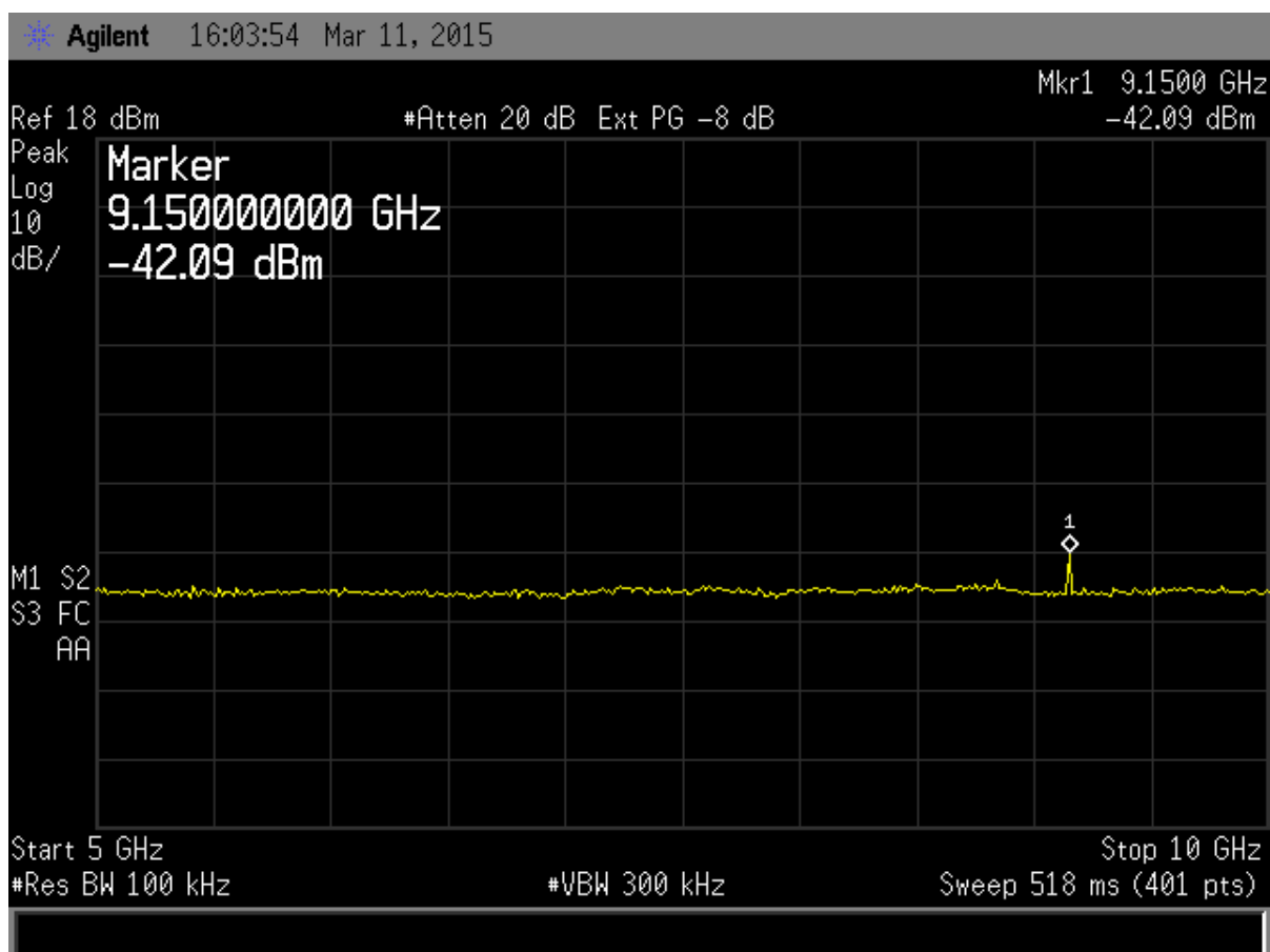
Figure 8. Antenna Conducted Emissions Mid, Part 3 GFSK Modulation
