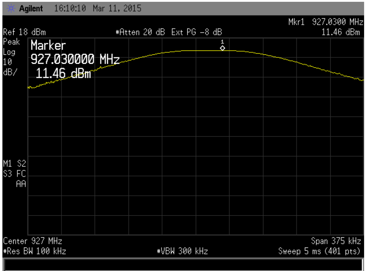
Figure 26. Peak Antenna Conducted Output Power, High Channel
