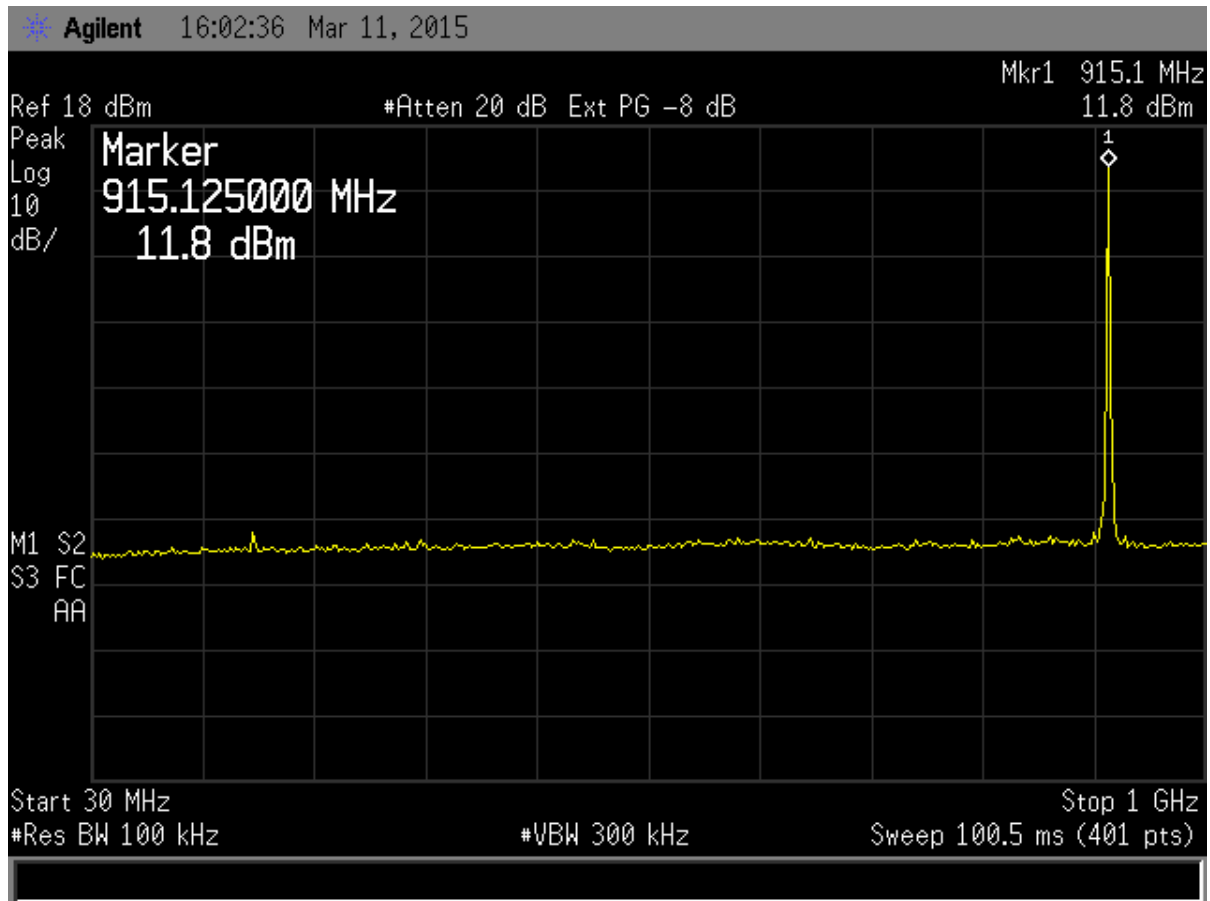
Figure 6. Antenna Conducted Emissions Mid, Part 1 GFSK Modulation
