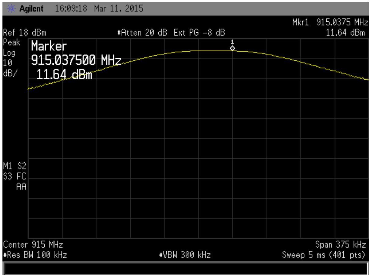
Figure 25. Peak Antenna Conducted Output Power, Mid Channel
