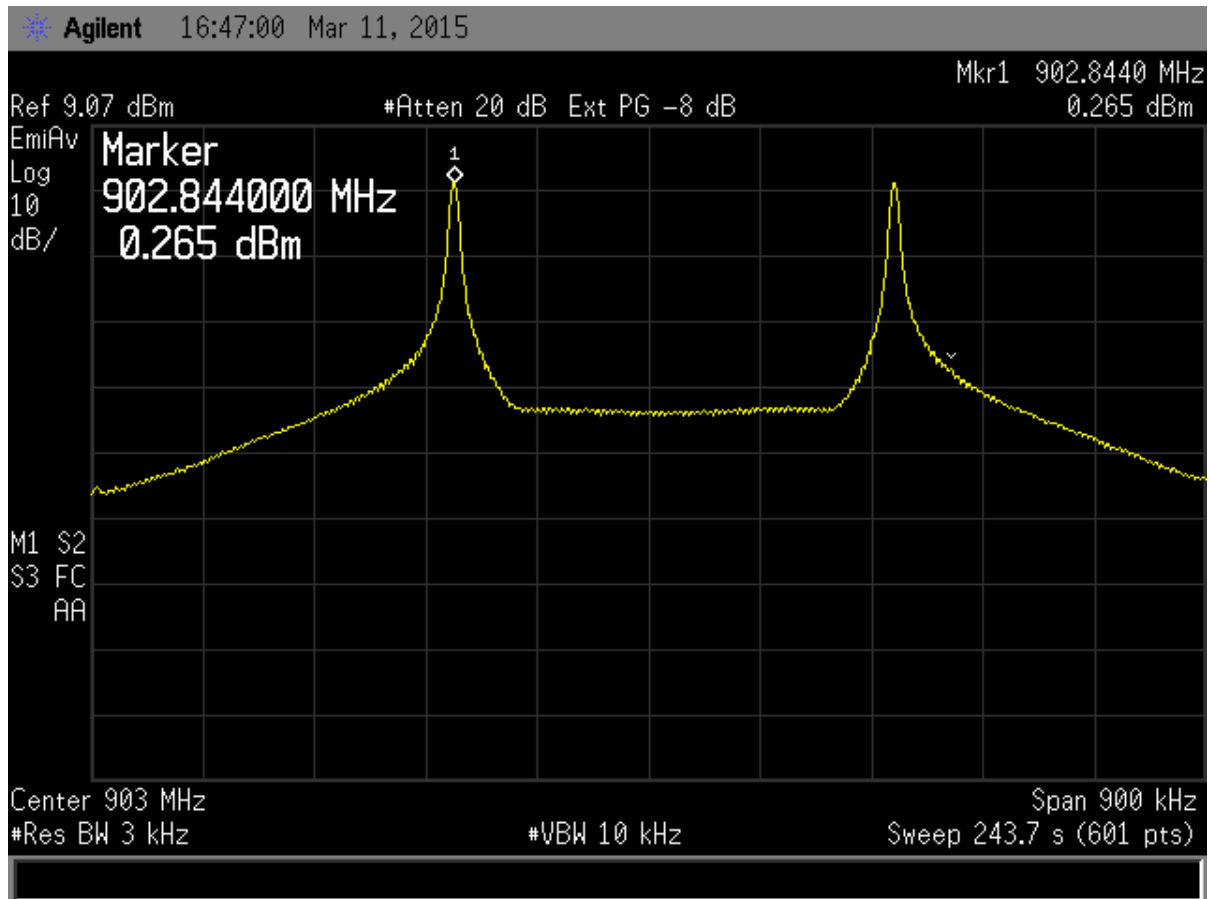
Figure 27. Peak Power Spectral Density, Low Channel
