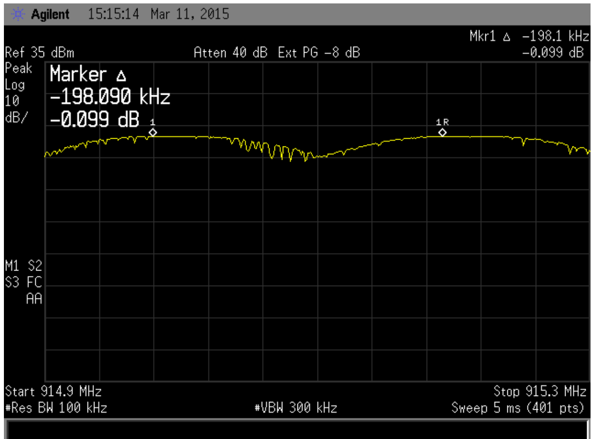
Figure 33. Channel Separation
