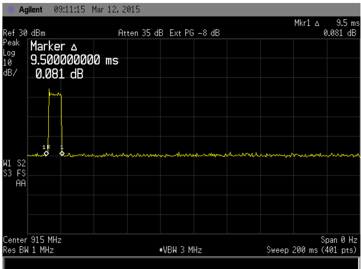
Figure 34. Time On
