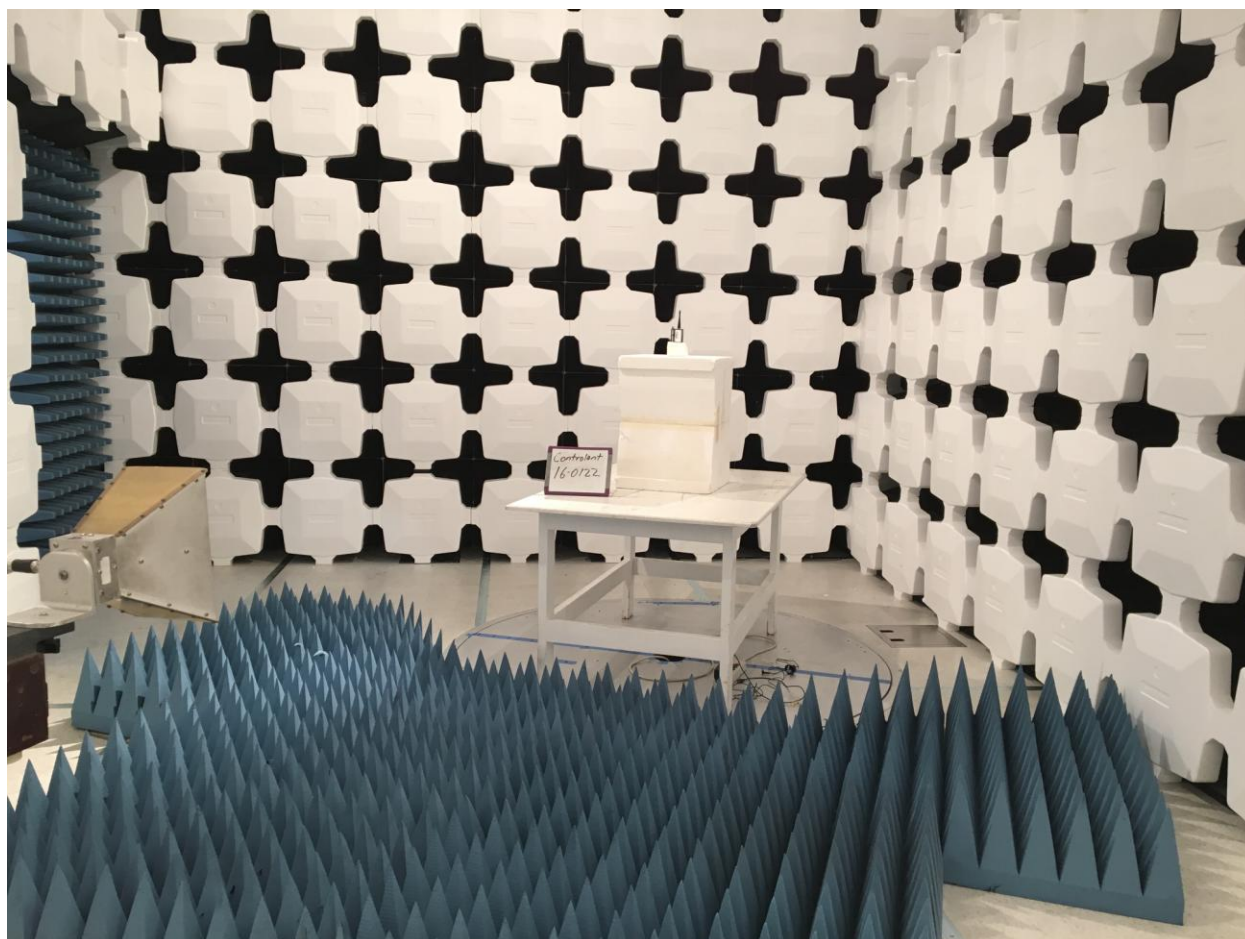
Figure 3. Radiated Emissions Test Setup – 1000 Mhz to 6 Ghz
