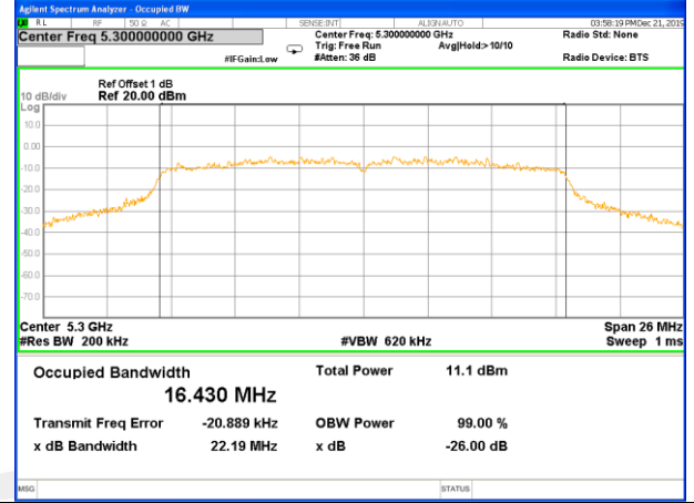
W53_11n20_Lower_26BW and 99%
