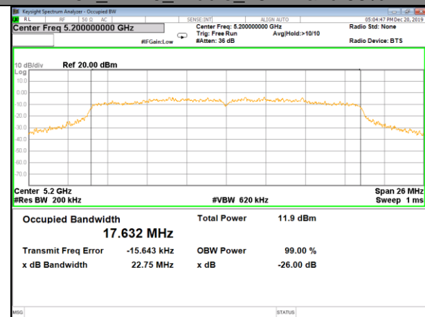
W52_11n20_Middle_26BW and 99%
