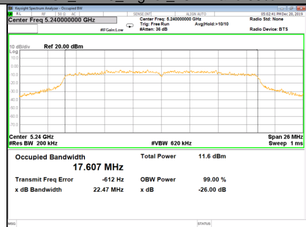
W52_11n20_Higher_26BW and 99%
