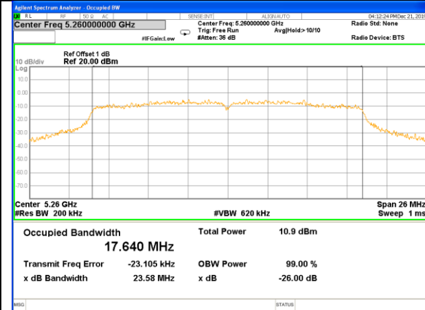
W53_11ac20_Higher_26BW and 99%
