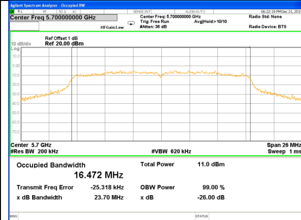
W56_11n20_Middle_26BW and 99%
