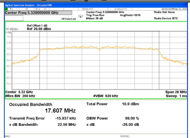
W53_11n20_Higher_26BW and 99%
