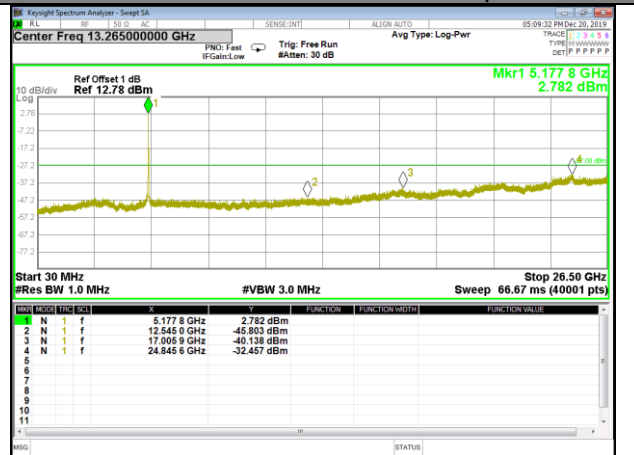
W52_11n20_Lower_Conducted Spurious
