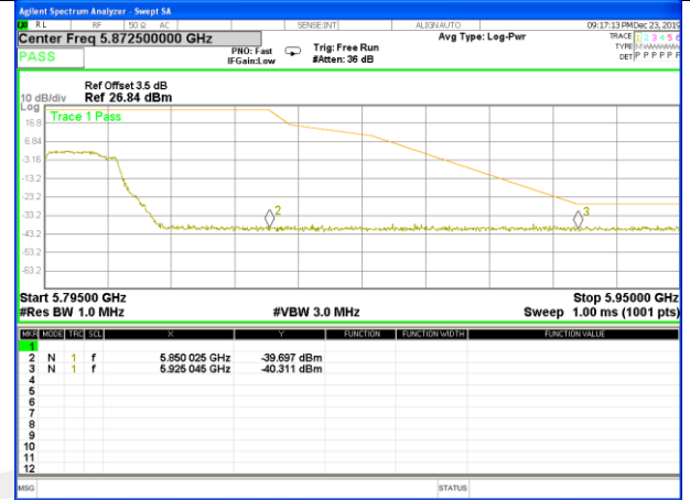
W58_11ac20_Middle_Conducted Spurious
