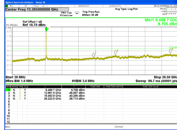
W56_11ac40_Higher_Conducted Spurious
