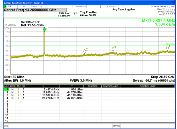
W56_11ac20_Higher_Conducted Spurious
