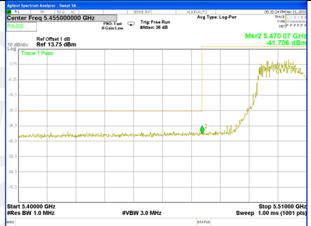
W56_11ac80_Lower_Conducted Spurious
