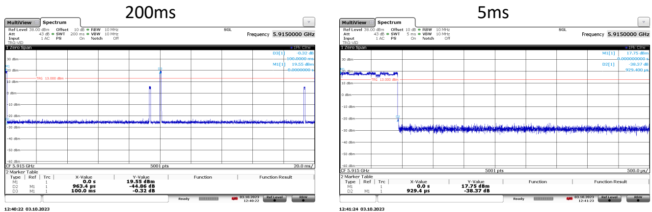
Figure 4.2.1 Example Pulsed Emission Characteristics (Duty Cycle).
