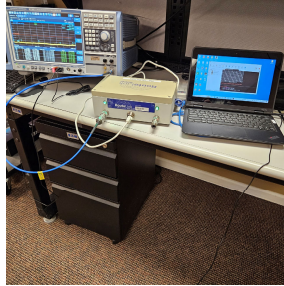
Figure 4.1.2 Conducted RF Test Setup Photograph(s).
