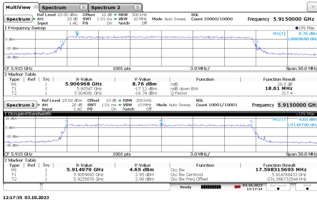
Figure 4.2.2 Example Intentional Emission Bandwidth.
