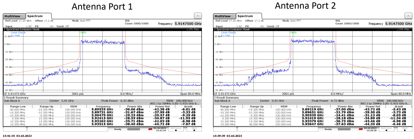
Figure 4.3.2 (i) Worst Case Transmitter OOBE Emissions Measured.
