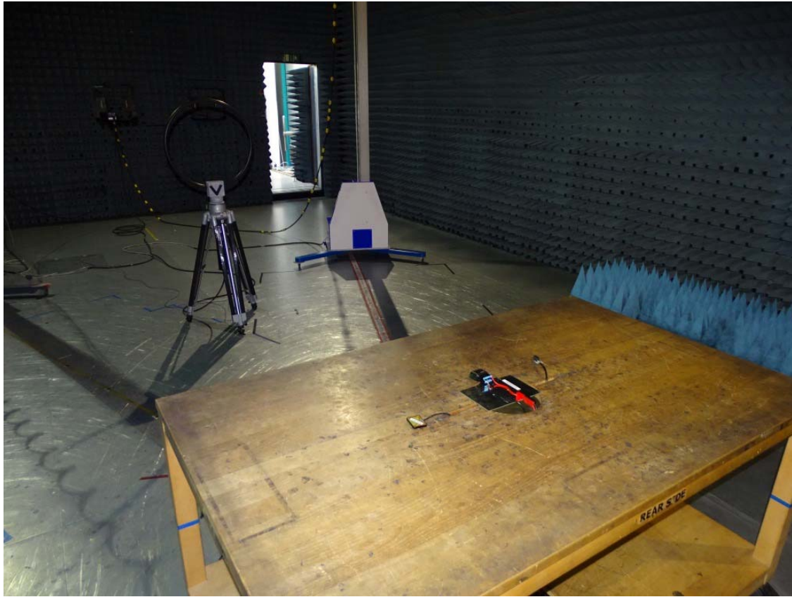
Photo 6: Test setup for radiated measurements (Enclosure, below 30 MHz, intentional radiator §15.209, ANSI C63.10)
