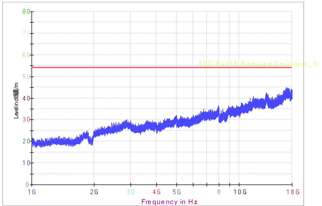
Plots No. 3: Radiated Band-Edge & Maximum Field Strength, Horizontal / Vertical Polarization
