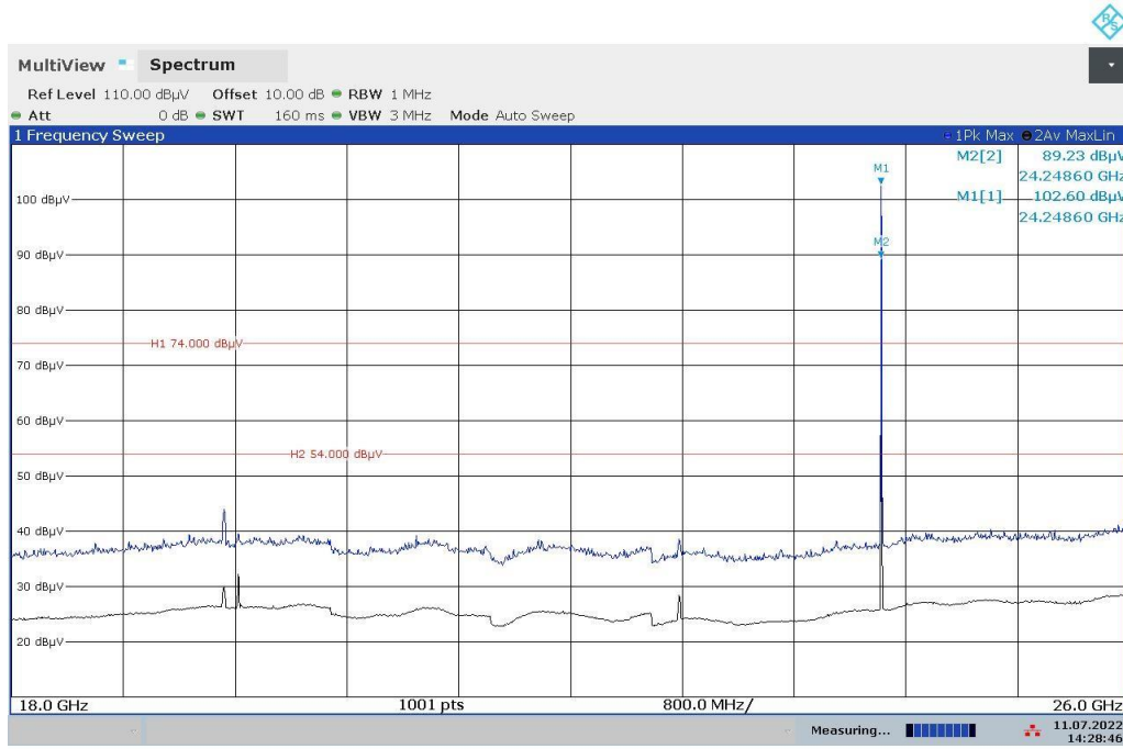
Plots No. 4: 18 GHz to 26 GHz, Horizontal / Vertical Polarization
