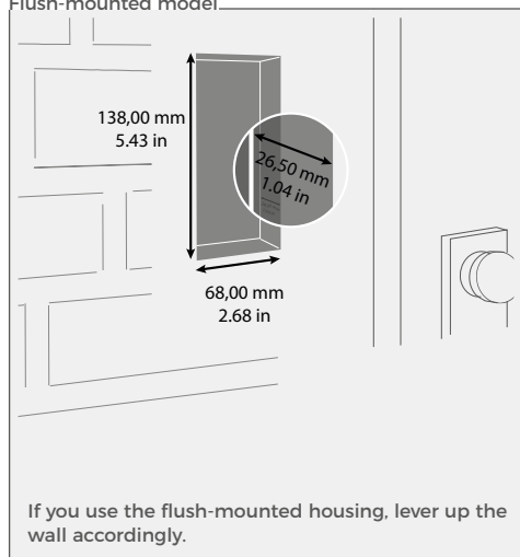
Flush-mounted model
