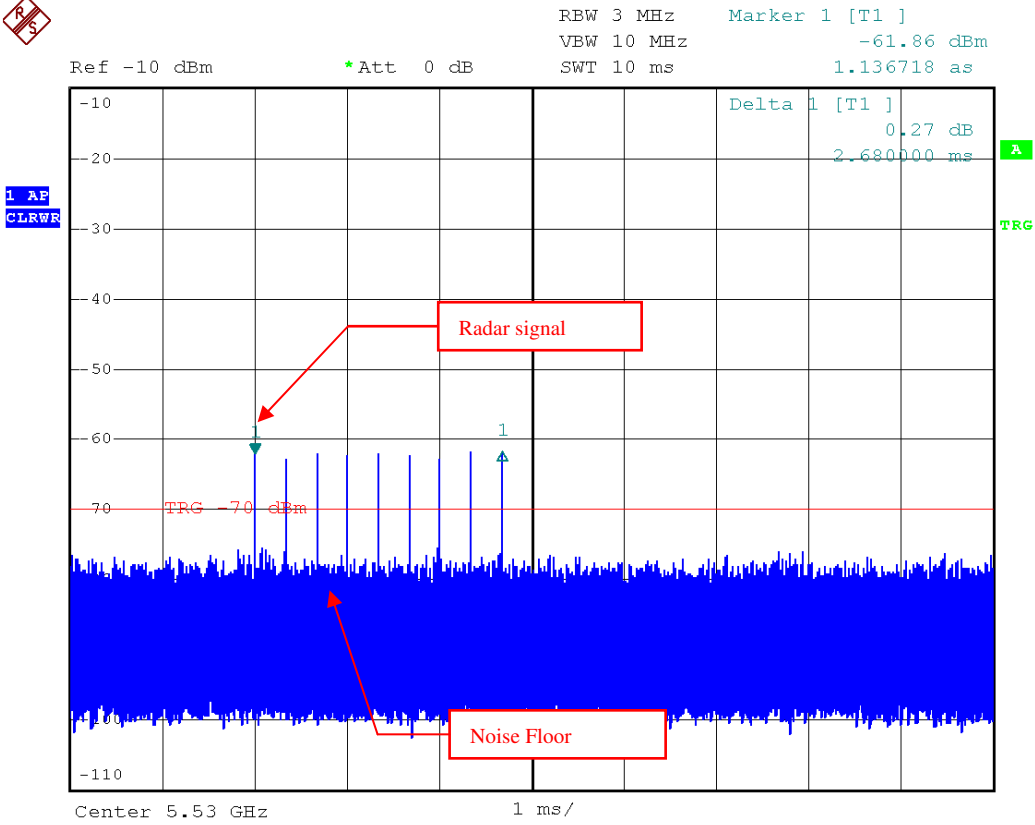
Radar Signal 6
