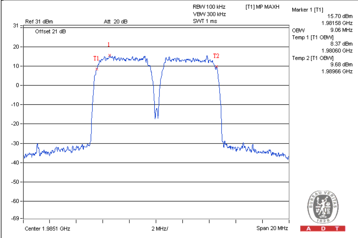
Spectrum Plot Of Worst Value WCDMA (CH 9913+9938)
