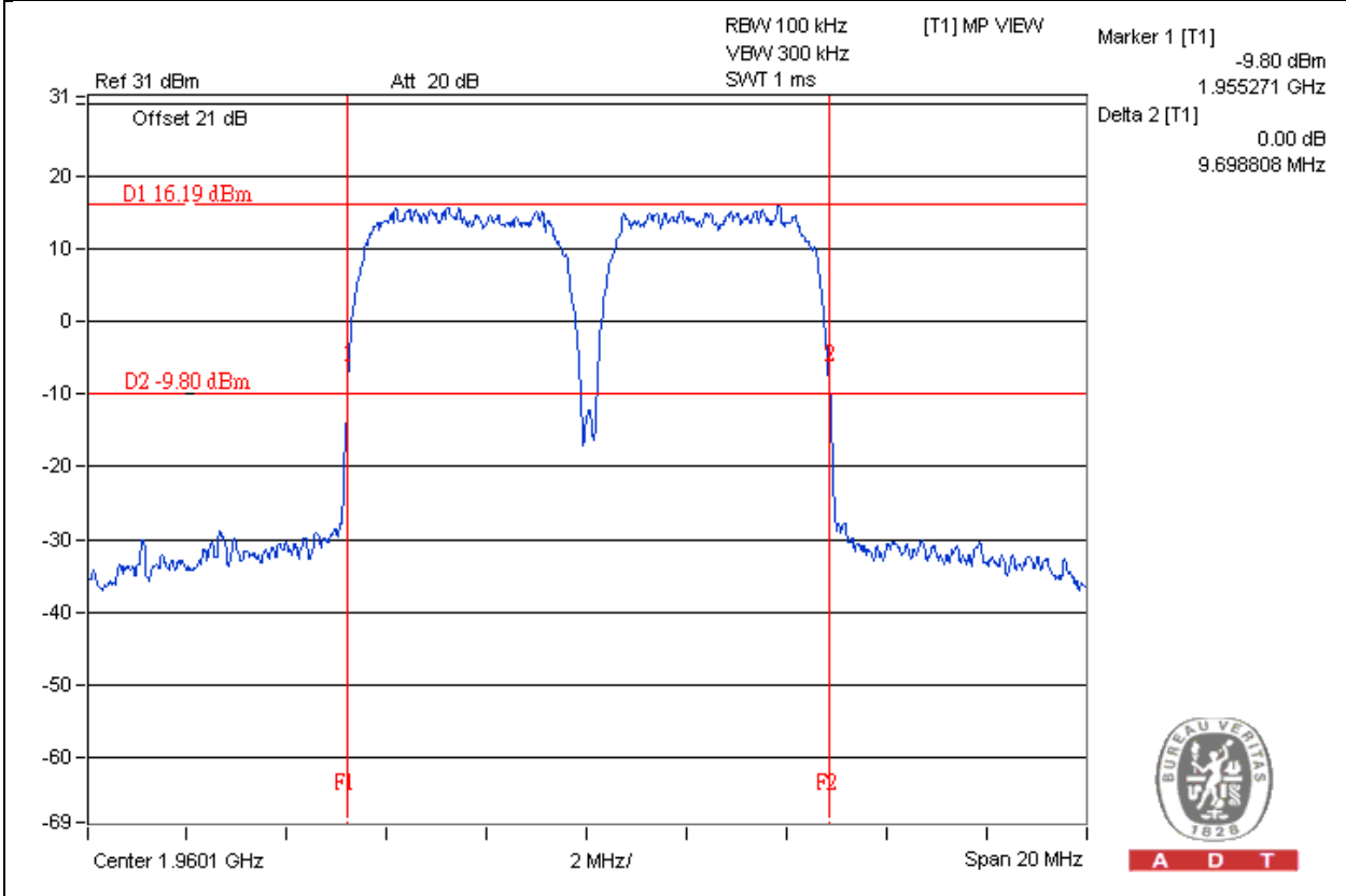
Spectrum Plot Of Worst Value WCDMA (CH 9788+9813)
