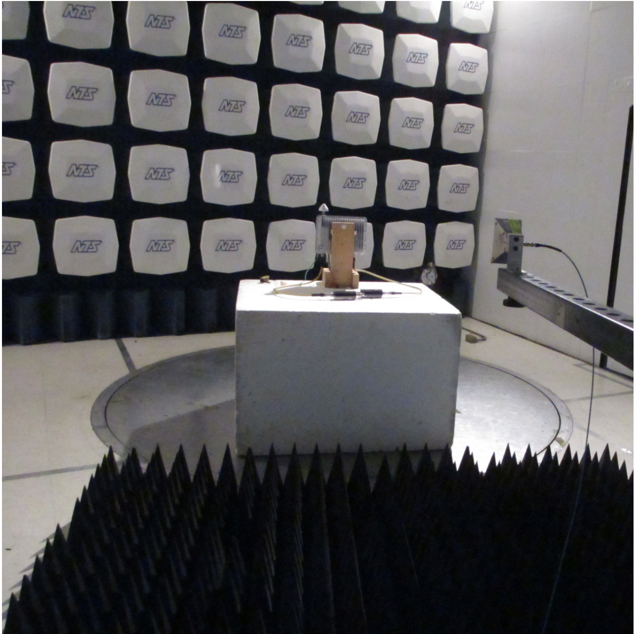
Radiated Emissions Setup – 18GHz to 27GHz
