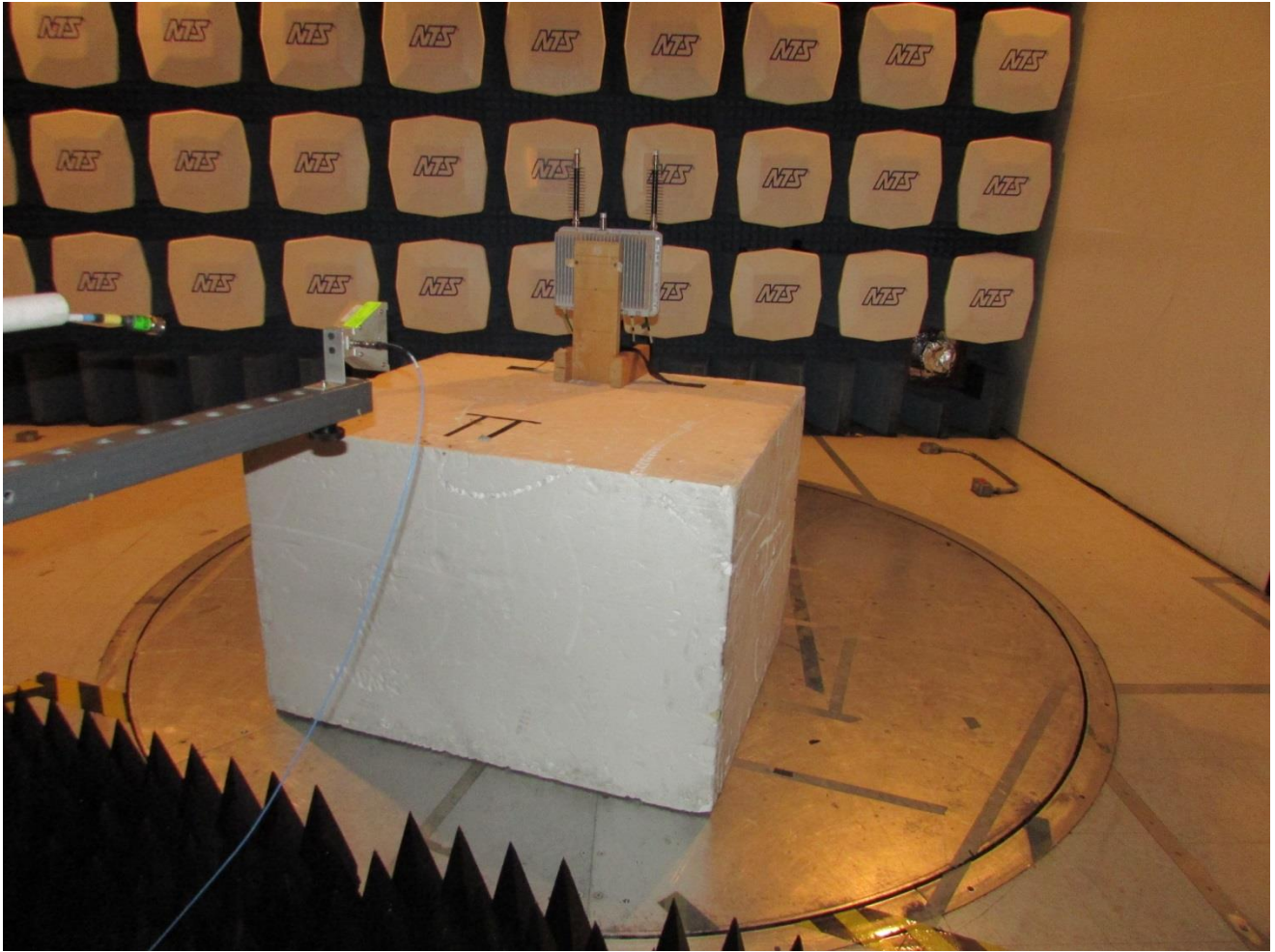
Radiated Emissions Setup – 18GHz to 27GHz
