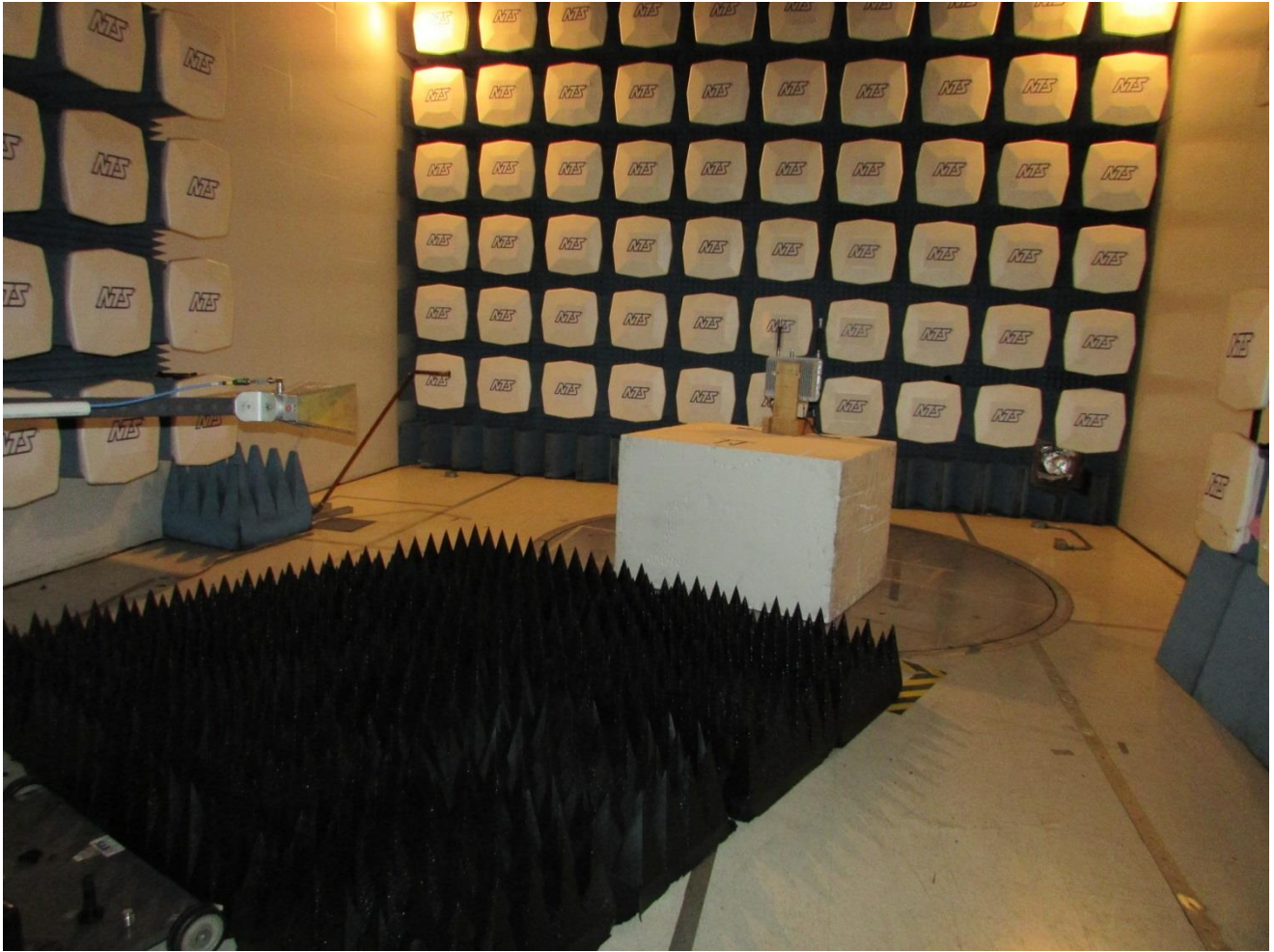
Radiated Emissions Setup – 1GHz to 10GHz
