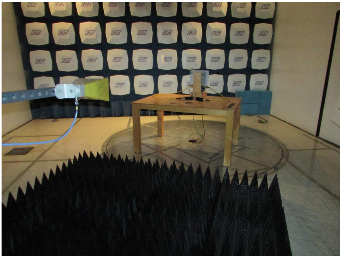
Radiated Emissions Setup – 1GHz to 18GHz
