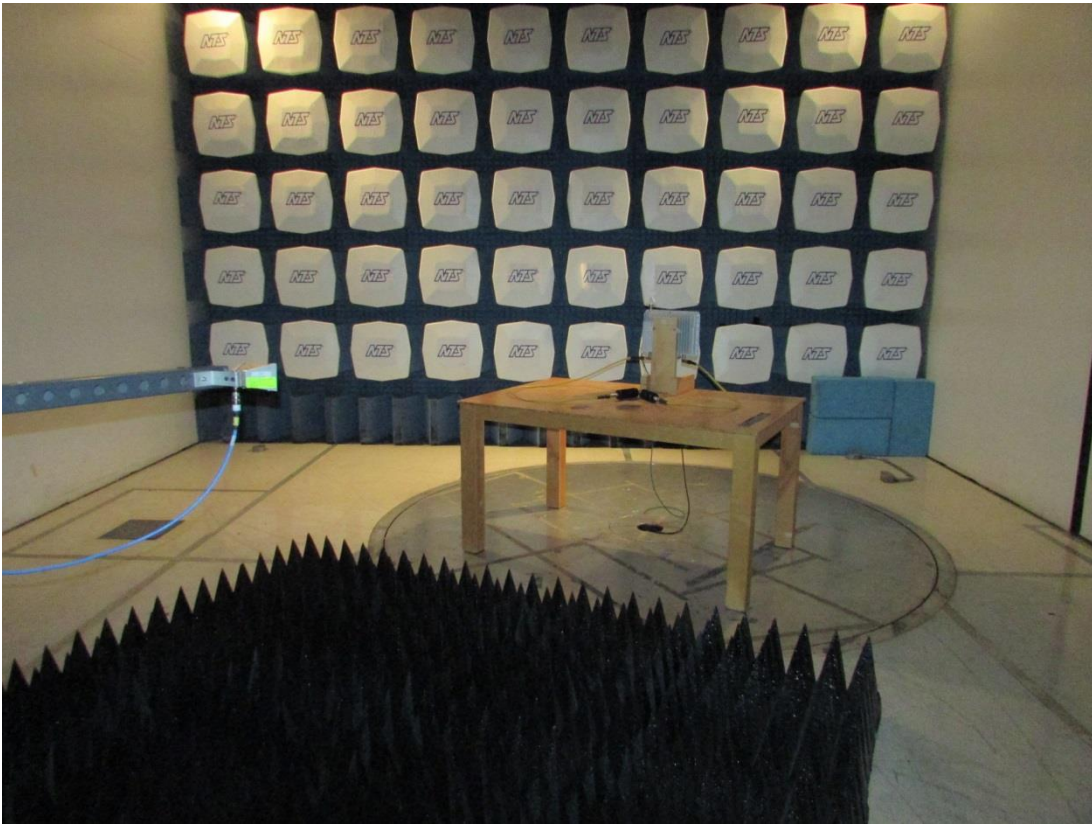
Radiated Emissions Setup – 18GHz to 20GHz
