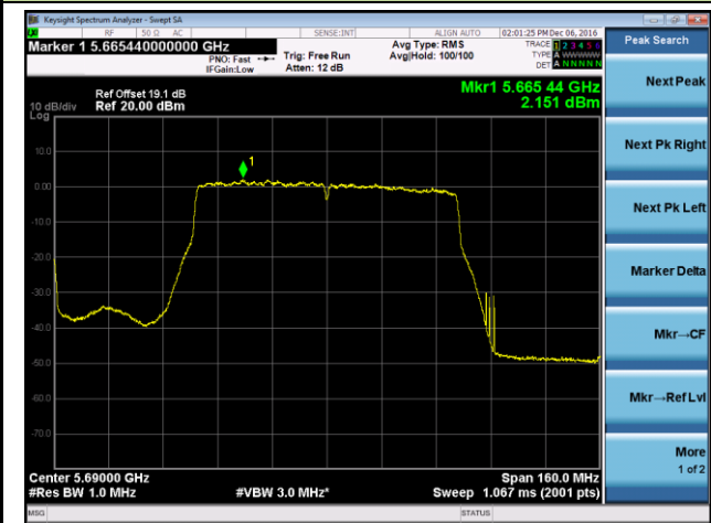
Channel 122+138 - Ant 2 (5690MHz)
