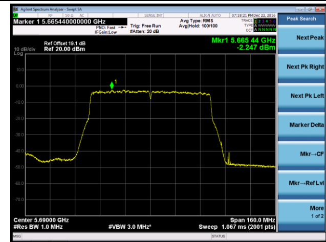
Channel 122+138 (5690MHz) - Ant 3
