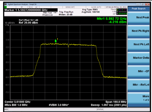
Channel 58+122 (5610MHz) - Ant 3
