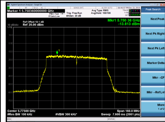
Channel 106+155 (5775MHz) - Ant 2
