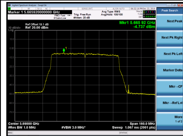
Channel 42+138 (5690MHz) - Ant 2
