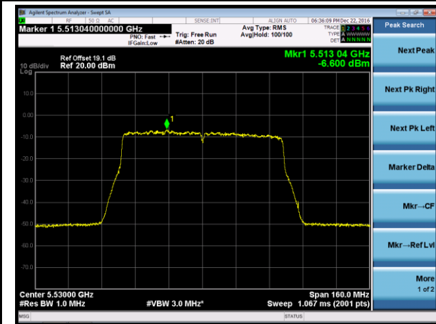
Channel 58+106 (5530MHz) - Ant 2
