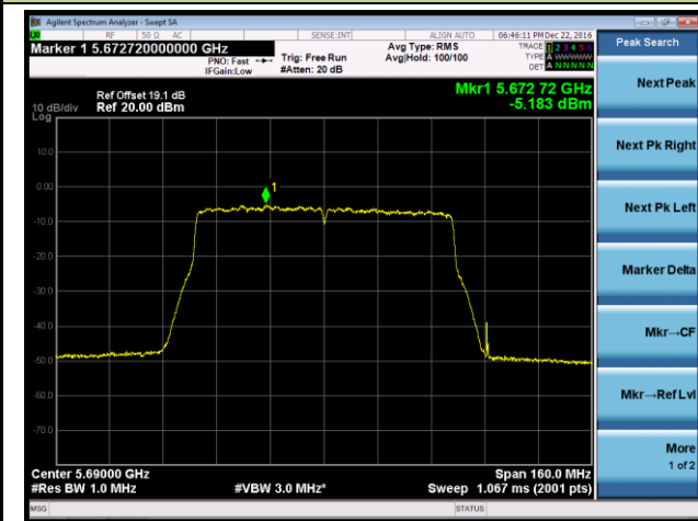
Channel 106+138 (5690MHz) - Ant 2
