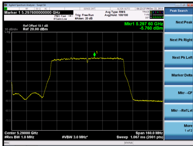
Channel 42+58 (5290MHz) - Ant 2
