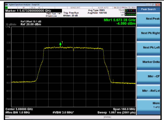
Channel 42+138 (5690MHz) - Ant 3
