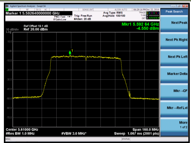
Channel 42+122 (5610MHz) - Ant 3
