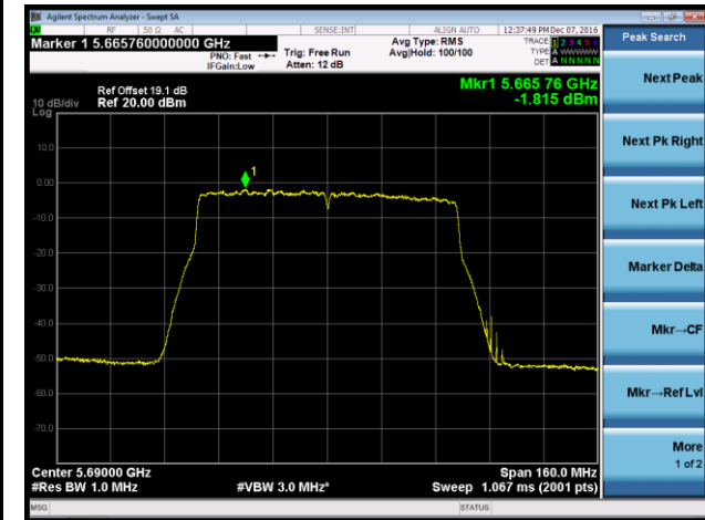
Channel 106+138 (5690MHz) - Ant 2
