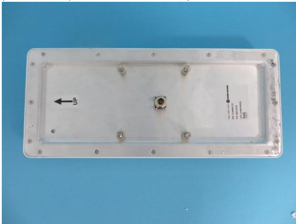
(12) Antenna Photo (Sector-Antenna 1356.17.0011)
