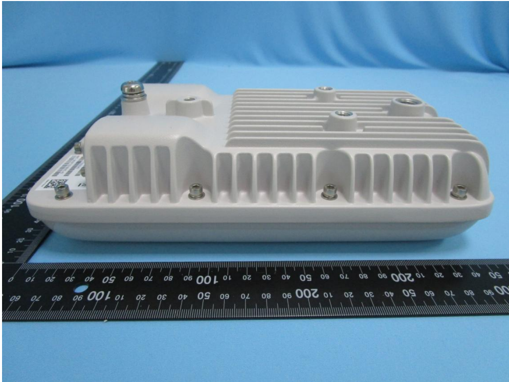
(5) External Photo - AC220 Wi-Fi AP OD directional antenna US (Side View)
