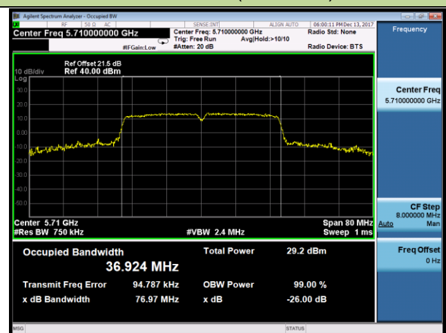
Channel 142 (5710MHz)
