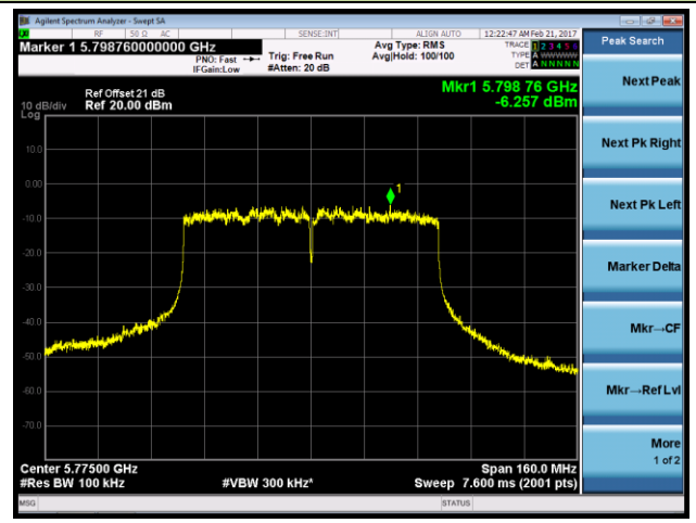
Channel 155 (5775MHz)
