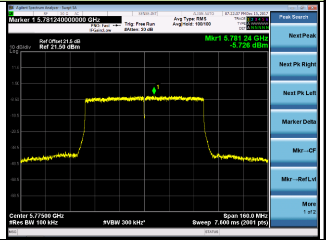
Channel 155 (5775MHz)
