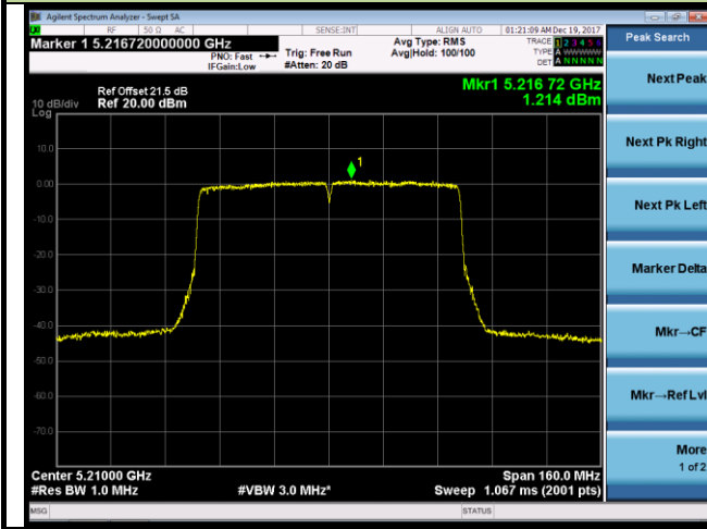
Channel 42 (5210MHz)
