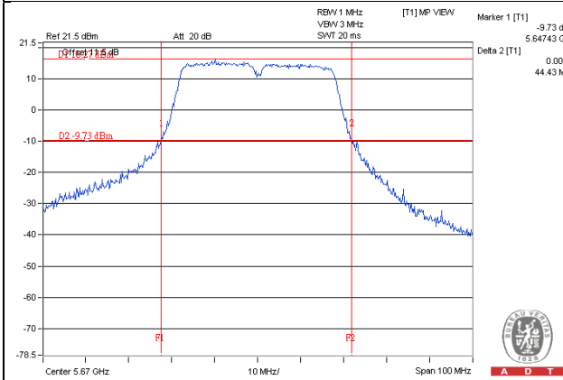
802.11ac (VHT40): Chain 1 / CH134
