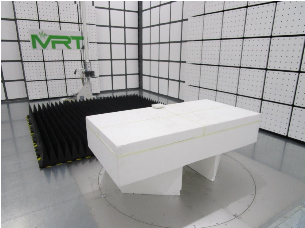
Description: Radiated Emission Test Setup for 1GHz ~ 18GHz (Test Mode 2)
