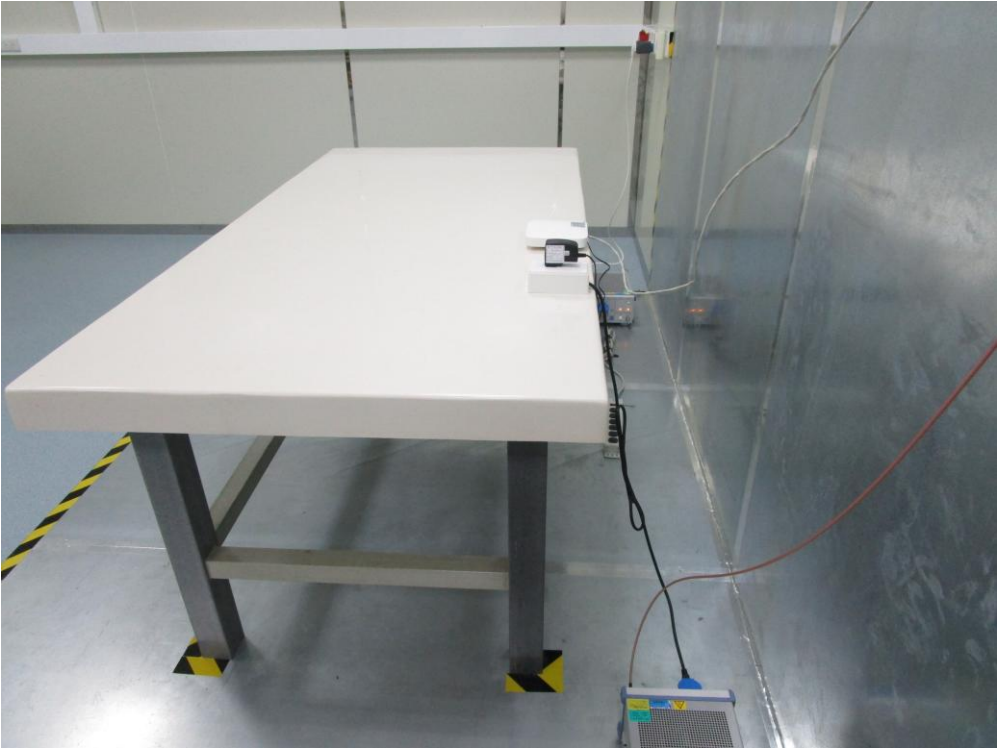
Description: Back view of Conducted Emission Test Setup (Test Mode 1)
