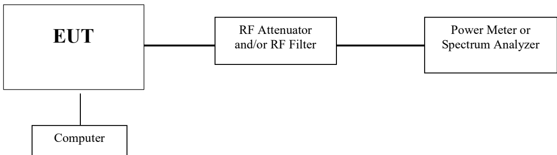
Figure 1. Setup Diagram of Conducted Test for RF Output Power, Power Spectrum Density, Occupied Bandwidth and Unwanted Emissions.
