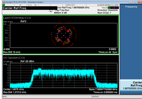
ModAnalysis_TM1_1_1C_5MBW_1987_TX1 IB_1987
