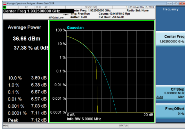
PAR_TM1_1_1C_5MBW_1932_TX1 IB_1932
