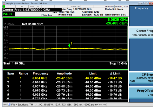
Spurious_TM1_1_1C_15MBW_1937_TX1_GB_1990_to_10000
