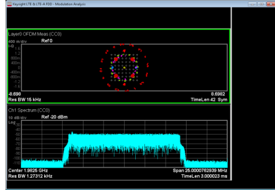
ModAnalysis_TM1_1_1C_15MBW_1982_TX1 IB_1982
