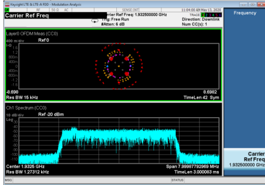
ModAnalysis_TM1_1_1C_5MBW_1932_TX1 IB_1932
