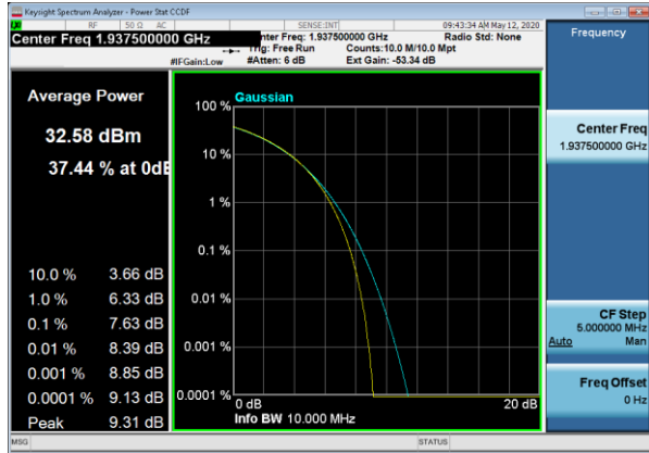
PAR_TM1_1_1C_15MBW_1937_TX1 GB_1937
