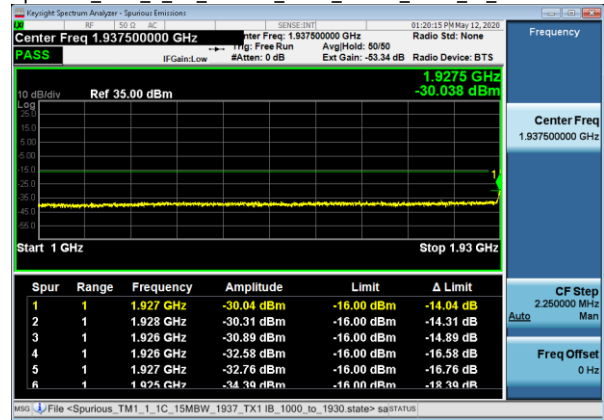
Spurious_TM1_1_1C_15MBW_1937_TX1 IB_1000_to_1930
