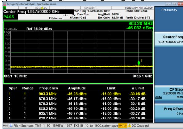
Spurious_TM1_1_1C_15MBW_1937_TX1 IB_10_to_1000
