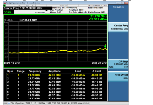
Spurious_TM1_1_1C_15MBW_1937_TX1_GB_10000_to_22000
