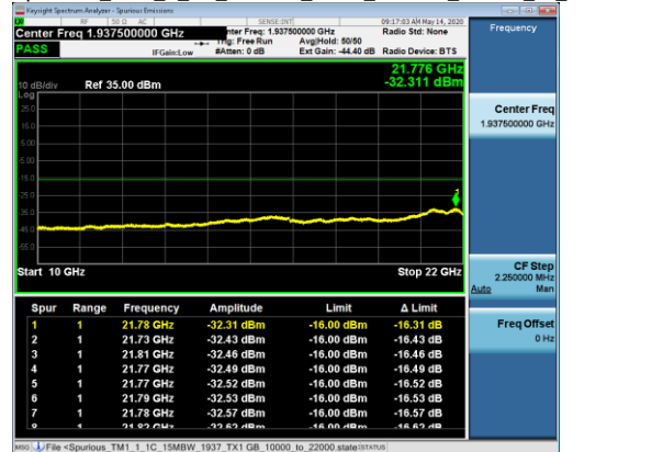
Spurious_TM1_1_1C_15MBW_1937_TX1 GB_10000_to_22000
