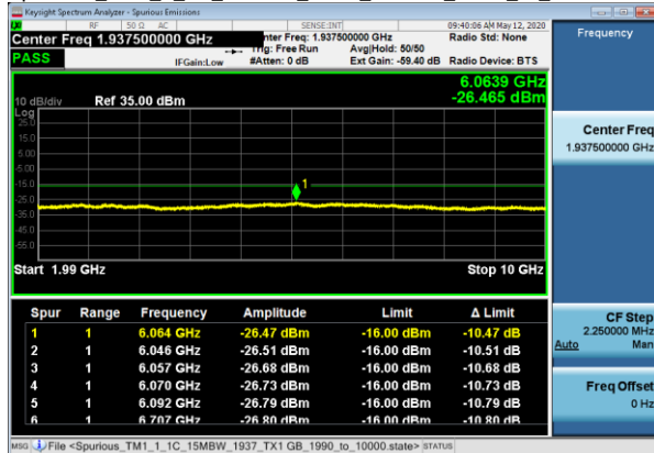
Spurious_TM1_1_1C_15MBW_1937_TX1 GB_1990_to_10000
