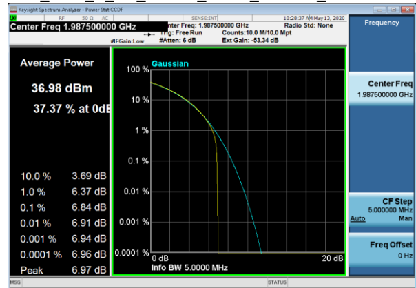
PAR_TM1_1_1C_5MBW_1987_TX1 IB_1987
