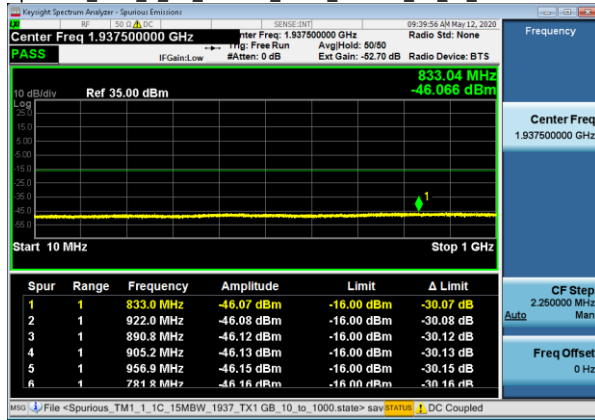
Spurious_TM1_1_1C_15MBW_1937_TX1_GB_10_to_1000
