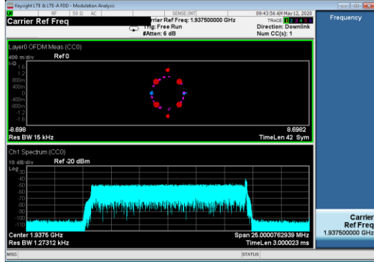
ModAnalysis_TM1_1_1C_15MBW_1937_TX1 GB_1937
