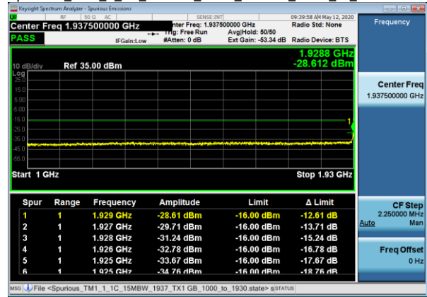
Spurious_TM1_1_1C_15MBW_1937_TX1_GB_1000_to_1930
