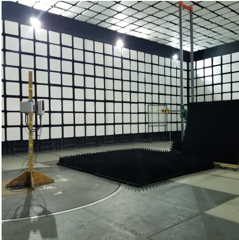
Radio Testing 18-33 GHz at 5.7m in AR-8
