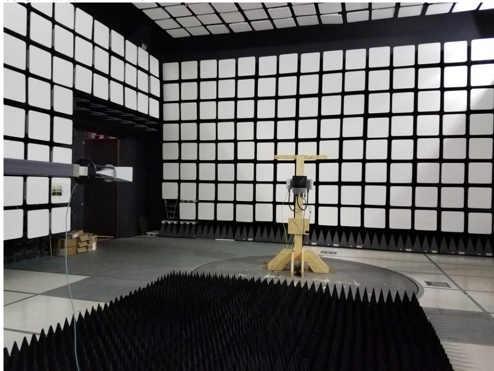
Radio Testing 18-33 GHz at 5.7m in AR-8
