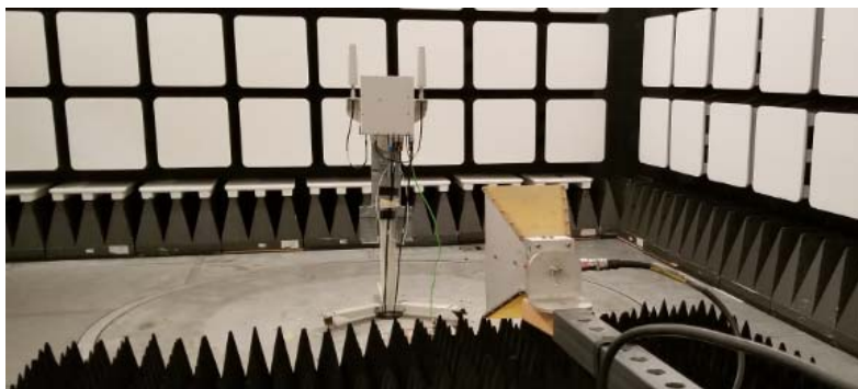
Figure 5. Setup Photos of Radiated Test for AZRB with Various Antennas (BA-AIO3O3T3T3VJX65F-06, PAS2457-CC1, GO4806-06664, 2205 & FA2RA)
